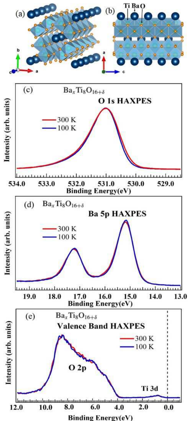
FIG. 1: (Color online) (a) Crystal structure of \text{BaTi}_8\text{O}_{16+\delta} [30] using VESTA [34] from tilted c -axis, (b) along ab plane. Ba, Ti, and O atoms are shown by filled circles with different colors. (c) HAXPES spectra of \text{Ba}_x\text{Ti}_8\text{O}_{16+\delta} at 300 and 100 K for O 1s , (d) Ba 5p , and (e) valence band.
