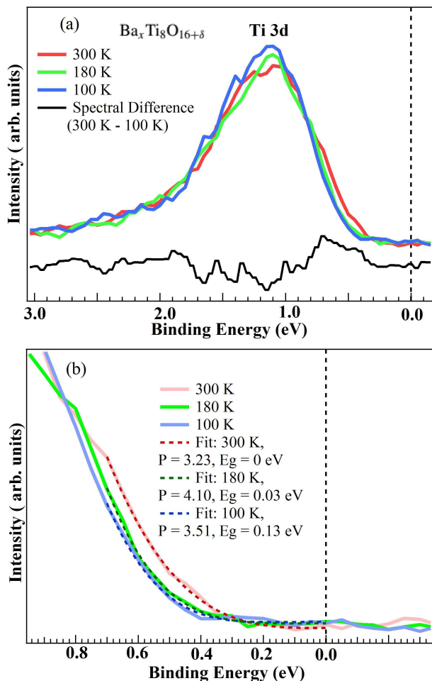
FIG. 3: (Color online) HAXPES spectra of \text{Ba}_x \text{Ti}_8 \text{O}_{16+\delta} at 300, 180, and 100 K (a) for Ti 3d area and (b) near the Fermi level.
