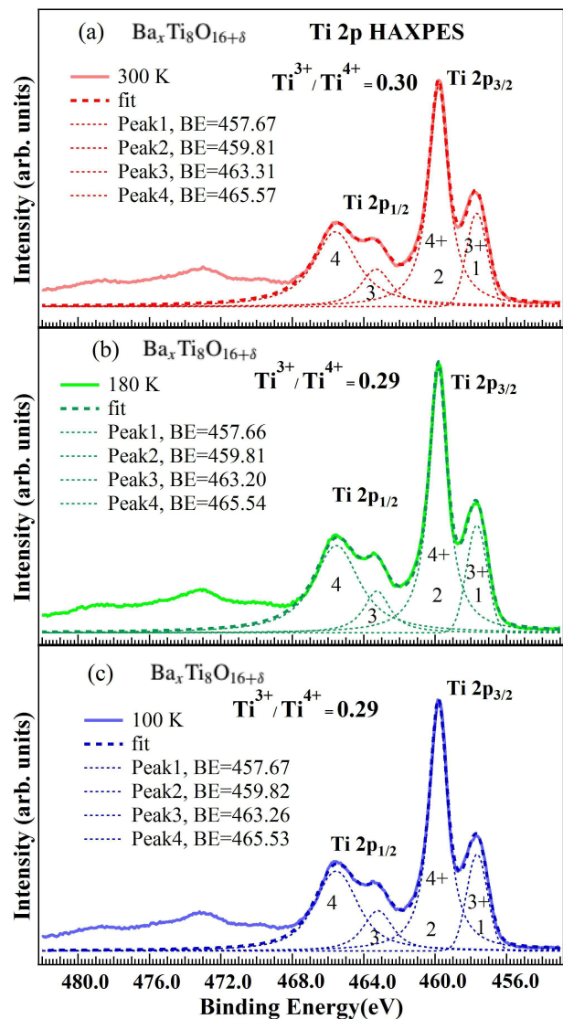
FIG. 2: (Color online) Ti 2p HAXPES spectra fitted with four Voigt functions for (a) 300, (b) 180, and (c) 100 K. Peak 1 and 2 represent for \text{Ti}^{3+} and \text{Ti}^{4+} components in the \text{Ti } 2p_{3/2} . Peak 3 and 4 are fitted for the \text{Ti } 2p_{1/2} region.
