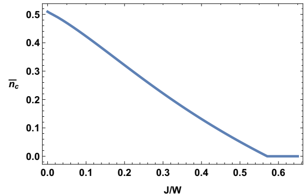
FIG. 1. The electron density \bar{n}_c below which the generalized Nagaoka state becomes unstable to a single spin flip. W = 8t is the band width for a 2D square band. When J/W is larger than a critical value around 0.57, a single spin flip is not sufficient to destabilize the state for any electron density.
