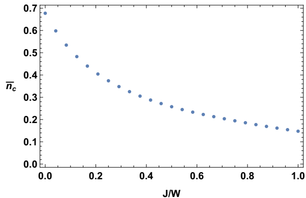
FIG. 2. The critical value of electron density \bar{n}_c below which the Nagaoka-like state |\psi_t^{3D}\rangle becomes unstable to a single spin flip. W = 12t is the band width for the 3D cubic bands. Unlike in the case of 2D bands, \bar{n}_c does not approach zero for finite J/W because the 3D density of states vanishes at low density limit.
