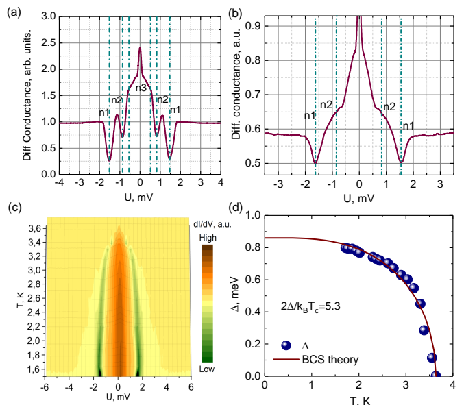
FIG. 4: (a) Dynamic conductance spectrum measured at T = 1.63 K for BaPd 2 As 2 single crystal with local critical temperature T_c = 3.75 K and for SnS Andreev contact with 3 Andreev reflections. (b) Dynamic conductance spectrum with 2 Andreev reflections at T = 1.63 K. Vertical green lines on panels a and b depict the dip positions. (c) Temperature evolution of conductance from the latter junction. (d) Temperature dependence of the obtained superconducting gap. Solid line shows a BCS-like curve for \delta .
