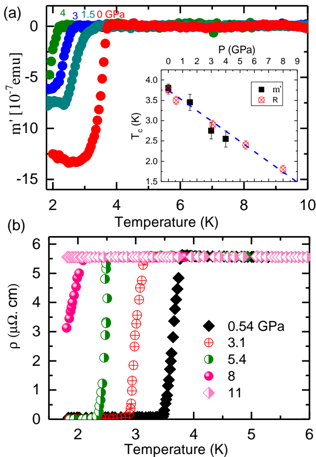
FIG. 5: Temperature dependence of magnetic moment of at different values of applied pressure. The inset shows the P-T phase diagram which illustrates the decrease of T_c with the applied pressure. (b) In-plane electrical resistivity of \text{BaPd}_2\text{As}_2 versus temperature showing the SC transition for different values of the applied pressure.
