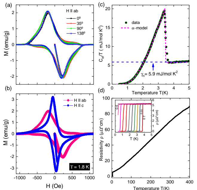
FIG. 2: (a) represents the identical values of magnetic moment with different in-plane angles. (b) shows the isothermal magnetization M vs. H loop at 1.8 K for H \parallel ab and H \parallel c . (c) illustrates the superconducting electronic specific heat c_{el} of \text{BaPd}_2\text{As}_2 as a function of the temperature (after subtracting the phonon contribution). The dashed line represents the theoretical curve based on single-band weak coupling BCS theory based on the \alpha -model. (d) presents the in-plane electrical resistivity \rho of \text{BaPd}_2\text{As}_2 versus temperature. the inset shows the superconducting transition for different values of applied field (0T, 0.05T up to 0.5T) down to 400 mK.
