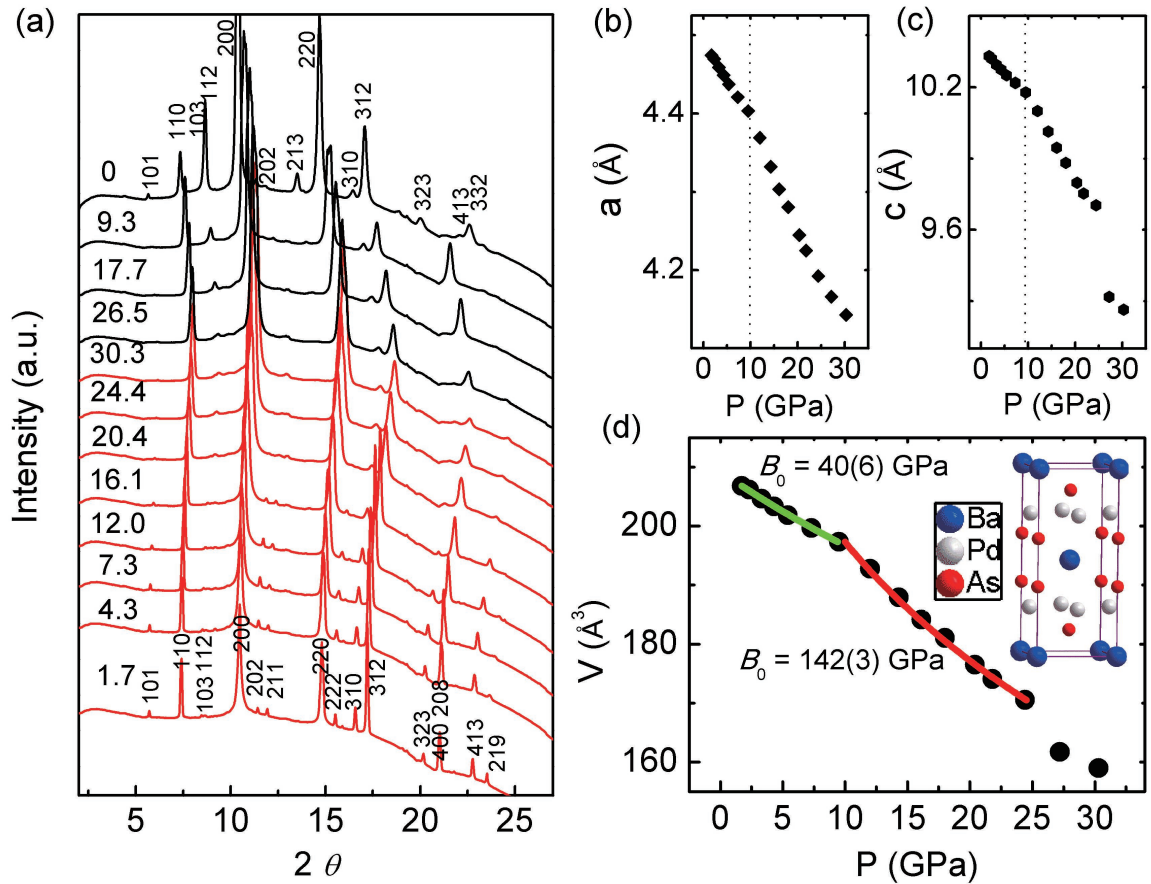
FIG. 8: (a) Angle-dispersive XRD patterns of BaPd 2 As 2 at selected pressures. The lattice parameters are shown in (b) and (c), obviously, both of the parameters a and c decrease faster with pressure above 9.5 GPa, while c shows a discontinuity at 27.2 GPa. In (a) The upper black patterns represent data at increasing pressure, while the lower red ones show data taken at decompression. (d) Unit cell volume obtained from Rietveld refinement of powder XRD patterns as a function of pressure. The inset shows its crystal structure.
