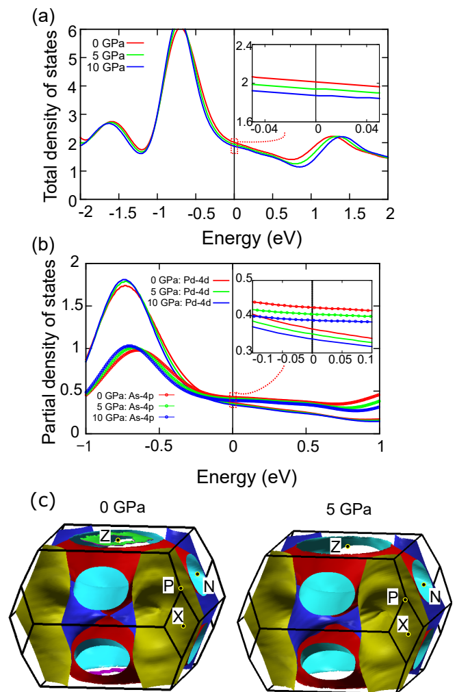
FIG. 6: (a) Total density of states (states/eV) of \text{BaPd}_2\text{As}_2 under pressures. (b) Pd-4d and As-4p partial densities of states (states/eV) under pressures. (c) The 3D Fermi surfaces in the Brillouin zone under pressures of 0 and 5 GPa. \text{BaPd}_2\text{As}_2 shows multi-band Fermi surface.
