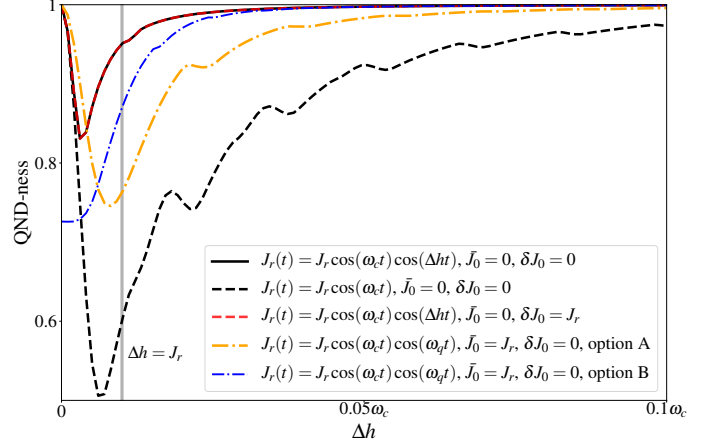
FIG. 2. As a figure of merit of the QND fidelity of the measurement process we use, for an initial excited state |+\rangle , i.e., \text{Min}[|\langle + | \langle + | \rangle]_\tau , and we take the maximum evolution time as \tau = 2/\kappa . Here we use parameters closer to those expected in a DQD-Cavity setup, with \omega_c/2\pi = 5 GHz, J_r/2\pi = 50 MHz and \kappa/2\pi = 25 MHz. In the black curve we set the static exchange tunneling to zero J_0 = 0 , and we tune \Delta h/2\pi across the range 0 to 250 MHz (the magnitude of J_r is indicated by the vertical gray line). The black dashed curve shows the same except with a modulation of the spin-photon coupling just at the cavity frequency alone. When \Delta h = 0 we recover the pure longitudinal result of Didier et al. 35 . As \Delta h is increased, the QND-ness of the two-tone modulation scheme decreases until a critical turning point, corresponding to the passage from an adiabatic regime to a fast-modulation regime, where the RWA starts to become valid. This regime is ideal when \Delta h = \omega_c/2 (see appendix for a complete analysis), but we see that, for the parameters in this example, it already performs well as \Delta h \rightarrow \omega_c/20 . The red dashed curve shows the influence of a modulated exchange tunnelling, \delta J_0/2\pi = J_r/2\pi = 50 MHz. The dashed orange curve shows the influence of a static exchange tunnelling, \bar{J}_0/2\pi = J_r/2\pi = 50 MHz, following the strategy A for preparation and readout, described in the text. The dashed-dotted blue curve shows the influence of a static exchange tunnelling, \bar{J}_0/2\pi = J_r/2\pi = 50 MHz, following the strategy B for preparation and readout, also described in the text. In the cases with static exchange coupling present, we modulate the spin-photon coupling at the eigenenergy of the dot system \omega_q = \sqrt{\Delta h^2 + \bar{J}_0^2} .
