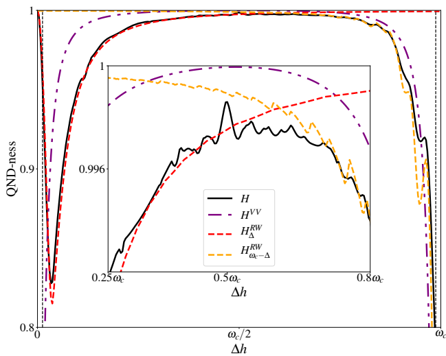
FIG. 4. As in Fig. 2, we plot the QND fidelity of the measurement process \text{Min}[\langle |+\rangle\langle +| \rangle]_{\tau} for an initial excited state |+\rangle as a function of \Delta h . In this figure we use larger coupling magnitude, J_r = 0.1\omega_c , and loss \kappa = J_r/2 , to accentuate the deviation from the ideal QND behavior. As before we choose the total integration time \tau = 2/\kappa . In black is the result for the full system Hamiltonian while the other lines correspond to the effective Hamiltonians listed in the table in the appendix. The black dashed vertical lines represent the points \Delta h = \{\tilde{J}_r, \omega_c - \tilde{J}_r\} , which set the boundary between the adiabatic and high-frequency regimes (which, for the reasons explained in the text, we expect to be valid in the long measurement time limit, i.e., when \kappa\tau \rightarrow \infty ). It is clear that operating at the point \Delta h = \omega_c/2 is optimal, as also suggested by our perturbative analysis, apart from the point corresponding to \Delta h = 0 , where the Hamiltonian is intrinsically longitudinal (corresponding to the proposal in reference [35]). The inset zooms on the parameter regime 0.2\omega_c < \Delta h < 0.8\omega_c .
