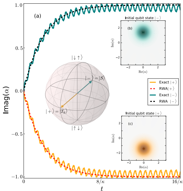
FIG. 1. (a) Shows an example of the evolution of the imaginary part of the cavity state \alpha = \langle a \rangle when the qubit is prepared in the \langle + \rangle or \langle - \rangle eigenstates of the \sigma_x for the two-tone modulated longitudinal readout scheme. Note that in our notation, the scheme is longitudinal in the \sigma_x basis, and is quasi-QND in that basis, as shown by the Bloch sphere inset. The dashed curves show the approximate RWA solution, while the solid lines show the full numerics, which includes oscillations due to the counter-rotating terms. The insets (b) and (c) show the Wigner function of the cavity state for the different initial qubit states at t = 16/\kappa . In this figure we have used non-ideal parameters to accentuate the unwanted oscillations, with \Delta h = 0.15\omega_c , J_r = 0.05\omega_c , and \kappa = J_r/2 . The oscillations due to counter-terms reduce the QND fidelity of the measurement, but this can be improved by of course increasing \Delta h or reducing the coupling strength J_r [and correspondingly reducing \kappa to maintain the same signal magnitude \alpha(t \rightarrow \infty) = J_r/2\kappa ].
