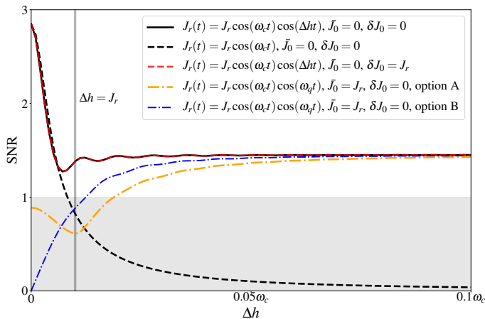
FIG. 3. Here we show the integrated signal-to-noise ratio obtained up to time \tau = 2/\kappa , as a function of \Delta h , with other parameters set as in Fig. 2, \omega_c/2\pi = 5 GHz, J_r/2\pi = 50 MHz and \kappa/2\pi = 25 MHz. The black curve shows that SNR is maximal for \Delta h \rightarrow 0 , then drops and saturates as \Delta h is increased (the magnitude of J_r is indicated by the vertical gray line). The black dashed curve shows the same except with modulation of the spin-photon coupling just at the cavity frequency alone. The red dashed curve shows the influence of a modulated exchange tunnelling, \delta J_0/2\pi = J_r/2\pi = 50 MHz. The dashed orange curve shows the influence of a static exchange tunnelling, \bar{J}_0/2\pi = J_r/2\pi = 50 MHz, following the strategy A for preparation and readout, described in the text. The dashed-dotted blue curve shows the influence of a static exchange tunnelling, \bar{J}_0/2\pi = J_r/2\pi = 50 MHz, following the strategy B for preparation and readout, also described in the text. In the cases with static exchange coupling present, we modulate the spin-photon coupling at the eigenenergy of the dot system \omega_q = \sqrt{\Delta h^2 + \bar{J}_0^2} .
