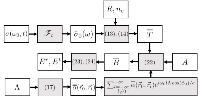
FIG. 4. The block diagram of the steps and equations involved in calculation of transmitted and reflected fields for a periodic array of wires wrapped by time-modulated graphene layers.
