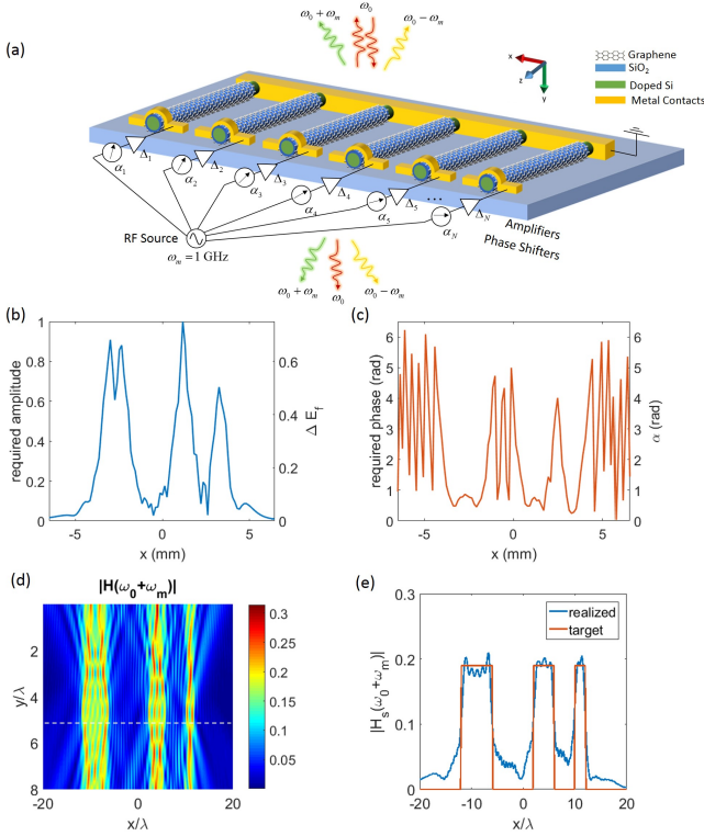
FIG. 8. Holographic generation of frequency harmonics using time-modulated metasurfaces. (a) The schematic of a time-modulated metasurface consisted of graphene-wrapped microwires biased via an active RF circuit incorporating amplifiers and phase shifters to provide required modulation depth and phase delay. (b) and (c) demonstrate the required amplitude and phase modulation at the metasurface plane, respectively which are mapped to the modulation depth and phase delay of the elements. (d) The magnetic field amplitude corresponding to the first-up modulated frequency harmonic generated in the forward direction (transmission). (e) Comparison of the ideal and realized patterns at the target plane located 5\lambda away from the metasurface plane.
