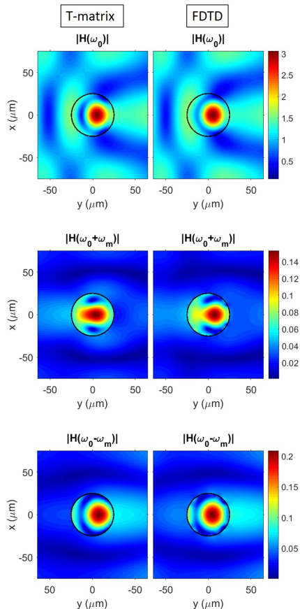
FIG. 5. The comparison of nearfield results obtained with the T-matrix and FDTD method corresponding to a periodic array of dielectric cylinders coated by sinusoidally modulated graphene layers incident normally by a TE-polarized plane wave.
