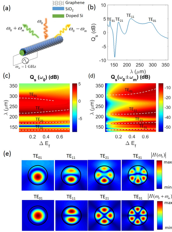
FIG. 6. Frequency conversion in a time-modulated graphene-wrapped microwire. (a) The schematic depiction of a graphene-wrapped Si/SiO 2 microwire modulated sinusoidally in time. (b) The TE scattering efficiency spectrum of time-invariant microwire with Fermi energy level of E_f = 0.3 \text{ eV} . The peaks correspond to TE resonant modes. (c) and (d) represent the scattering efficiencies of the fundamental and first-order generated frequency harmonics as functions of Fermi energy modulation depth and wavelength. (e) The profiles of magnetic field corresponding to the resonant modes of the fundamental and first-order frequency harmonics.
