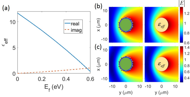
FIG. 9. (a) The effective permittivity of the deeply subwavelength graphene-wrapped microwire as a function of Fermi energy level of graphene. (b) and (c) compare the nearfield distributions of electric field corresponding to graphene-wrapped microwires and homogenized counterparts for Fermi energy levels of E_f = 0.2 eV and 0.5 eV, respectively.
