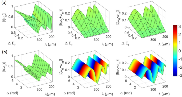
FIG. 7. (a) The amplitude and phase shifts of transmission coefficients corresponding to fundamental and first-order frequency harmonics as functions of wavelength and modulation depth of Fermi energy for a modulation phase delay of \alpha = 0 . The phase shift is depicted as pseudo-color and is measured at each wavelength with respect to the phase at \Delta E_f = 0 . (b) demonstrates the same as functions of wavelength and modulation phase delay of Fermi energy for a modulation depth of \Delta E_f = 0.75 . The phase shift at each wavelength is measured with respect to the phase at \alpha = 0 .
