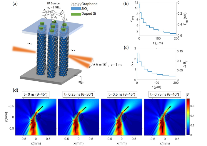
FIG. 10. Spatiotemporal manipulation of light using a time-modulated metamaterials. (a) The schematic depiction of a space-time gradient metamaterial consisted of graphene-wrapped microwires biased from the top using an RF biasing grid incorporating amplifiers to provide required modulation depth and offset for each element. (b) and (c) demonstrate the required average value and modulation depth of the effective permittivity, respectively as functions of radial position within the lens which are mapped to the average value and modulation depth of Fermi energy of graphene-wrapped microwires. (d) The steady-state electric field amplitude distribution at different time steps within a scanning cycle.
