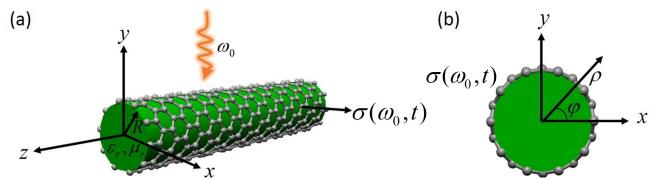
FIG. 1. The schematic of an isolated microwire wrapped by a time-varying graphene.
