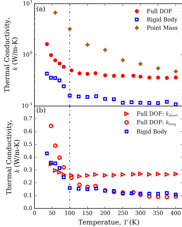
FIG. 5: (a) Thermal conductivity of the three C_{60} models plotted as a function of temperature. (b) Full DOF model thermal conductivity decomposition into k_{short} and k_{long} and comparison with the rigid body model. The error bars are smaller than the marker size. The vertical dash-dot line a temperature of 100 K.
