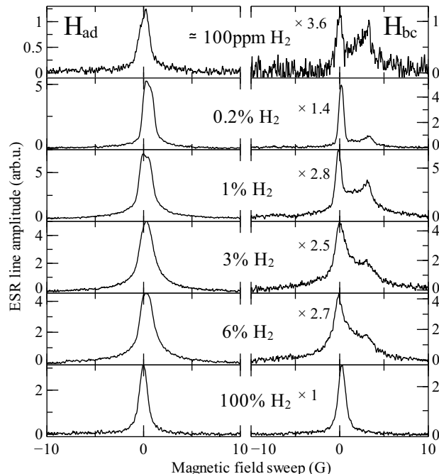
Figure 4. The H ad and H bc ESR lines measured in neon samples with different admixtures of H 2 studied in this work. Note that the H bc line amplitudes are multiplied by a factor specified for each plot. The distance between the lines is \approx 507 G.
