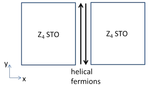
FIG. 2. Gapping out the helical fermions by a Z_4 STO.
