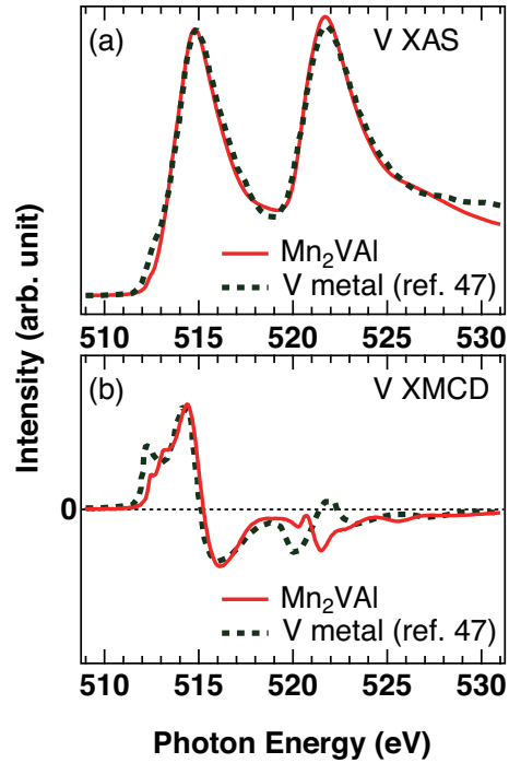
FIG. 5: (Color online) V L_{2,3} -edges XAS (a) and XMCD (b) spectra for \text{Mn}_2\text{VAI} (solid line) and V metal (dashed line) reported in the reference 47 . The XMCD spectra are normalized at the L_3 peak.
