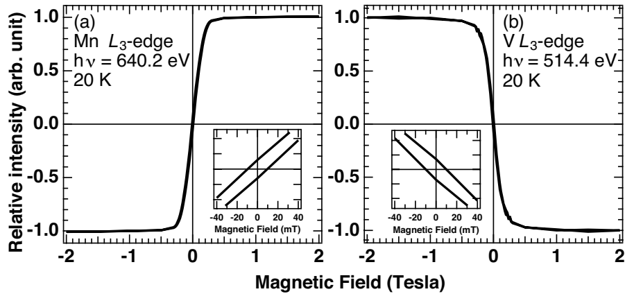
FIG. 3: (Color online) (a), (b) Magnetic field dependence of the XMCD intensity at the Mn and V L 3 peak. The inset shows the expanded view around the 0 T.
