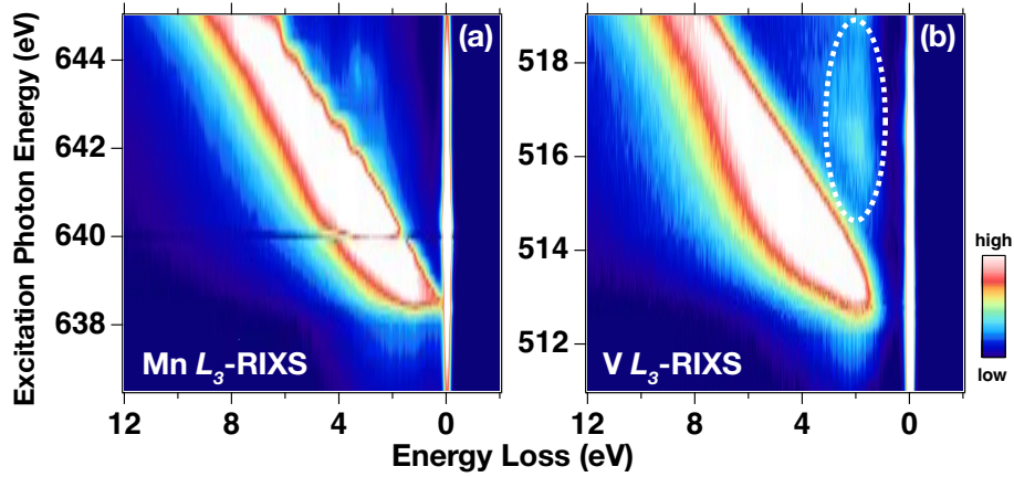
FIG. 8: (Color online) Intensity plots of h\nu_{in} -dependent RIXS at the Mn (a) and V (b) L -edges. Spectra are normalized by the photon flux. Dashed circle is the guide for the eye indicating the resonant excitation.
