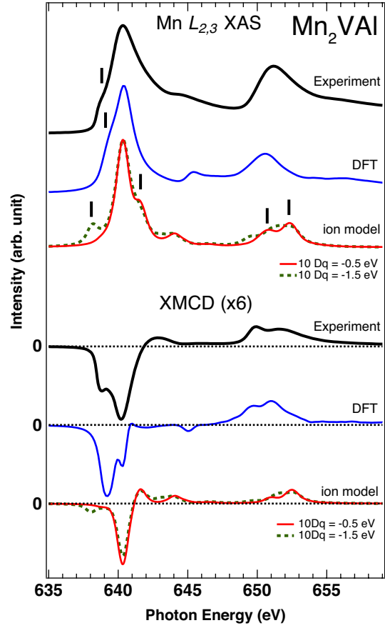
FIG. 6: (Color online) Mn L_{2,3} -edge XAS and XMCD spectra compared with the simulation based on DFT and the ionic model. Spectra are normalized by the L_3 -peak intensity of the polarization summed XAS spectra.
