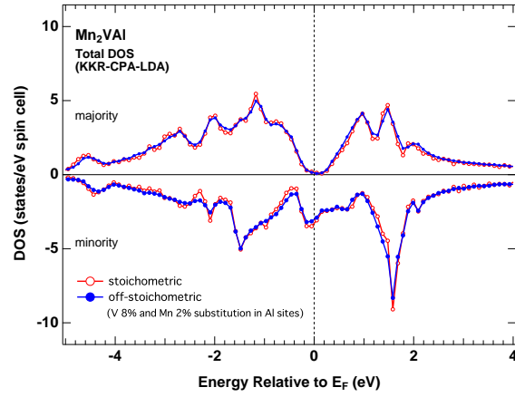
FIG. 9: (Color online) Off-stoichiometric effects on total density of states of Mn 2 VAI obtained by the KKR-CPA-LDA method.
