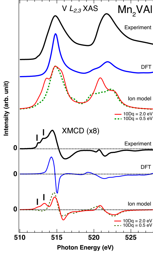
FIG. 7: (Color online) V L_{2,3} -edge XAS and XMCD spectra compared with the simulation based on DFT and the ionic model. Spectra are normalized by the L_3 -peak intensity of the polarization summed XAS spectra.
