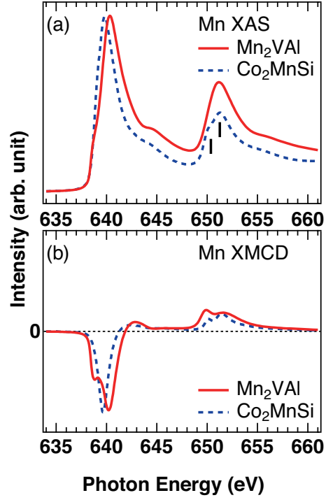
FIG. 4: (Color online) Mn L_{2,3} -edges XAS (a) and XMCD (b) spectra for \text{Mn}_2\text{VAI} (solid line) and \text{Co}_2\text{MnSi} (dashed line).
