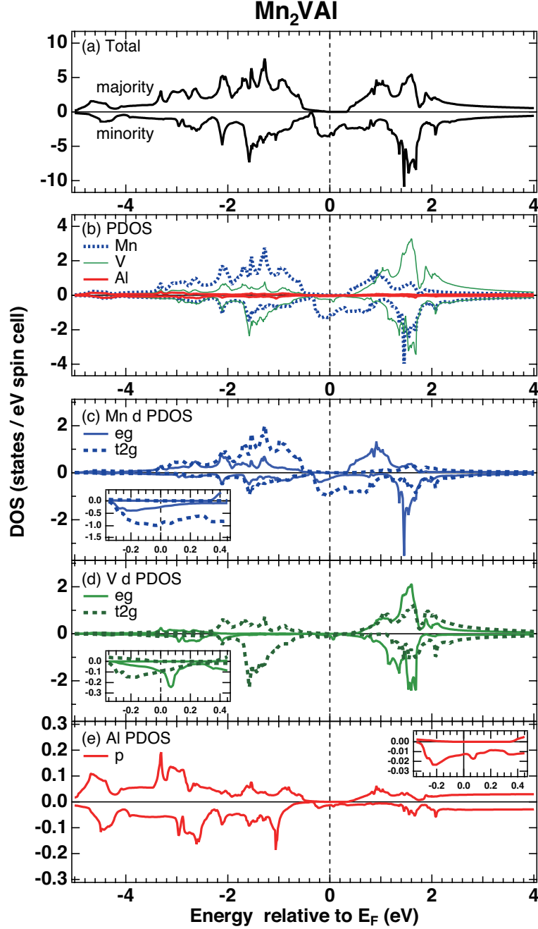
FIG. 1: (Color online) (a) Total density of states of L2 1 ordered Mn 2 VAI. (b) PDOS of Mn, V, Al sites. (c), (d) PDOS of Mn and V 3d states projected onto the e_g and t_{2g} orbital. (e) PDOS of Al 3p states. The insets show the enlarged view of PDOS around E_F .
