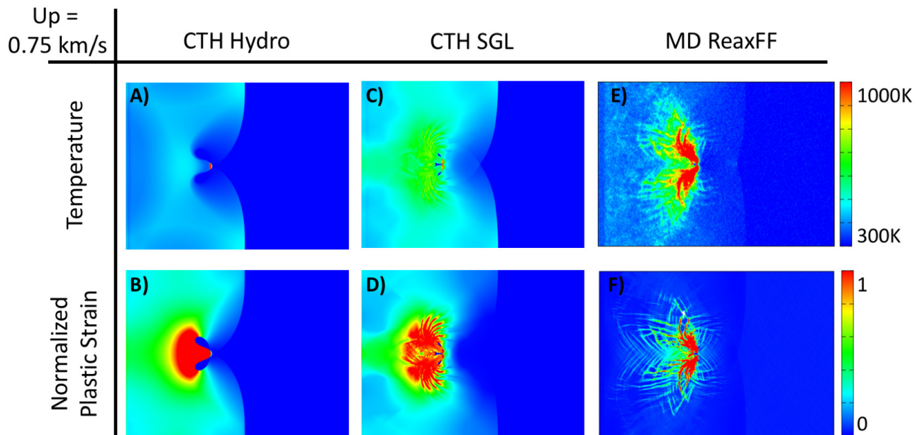
Figure 5. Comparison of the U_p = 0.75 km/s shock response of porous HNS for a single 0.1 \mu\text{m} pore. The temperature predictions from the CTH hydro model in regions of high plastic strain are noticeably colder than the strain rate dependent SGL model, which better captures the correlation of strain and temperature observed in the MD simulations.
