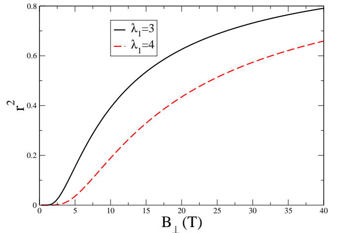
FIG. 3: r^2 vs. B_\perp for \lambda_1 = 3 and \lambda_1 = 4 . Note that r^2 tends vary rapidly to zero when B_\perp falls below a characteristic scale set by \lambda_1 . At large values of B_\perp , r^2 \rightarrow 1 . The approach to r^2 = 1 is very slow.
