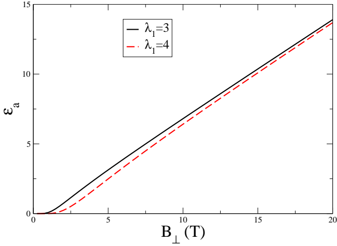
FIG. 4: Orbital anisotropy energy \epsilon_a vs. B_\perp for \lambda_1 = 3 and \lambda_1 = 4 . At very small values of B_\perp below a characteristic scale set by \lambda_1 , \epsilon_a vanishes rapidly as B_\perp \rightarrow 0 . At large values of B_\perp , \epsilon_a becomes linear in B_\perp .
