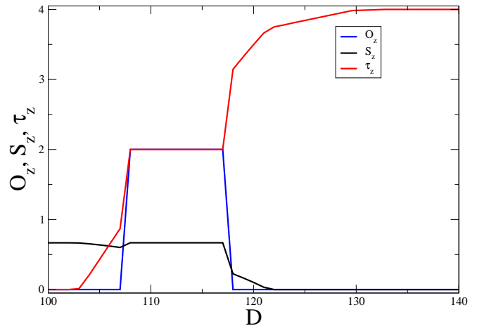
FIG. 7: Order parameters at B_{\perp} = 16\text{T} for PS1 with purely perpendicular field. Once again, the system is in the CAF state for small D . At around D = 102 , there is a second-order transition into the \text{BU}(1)^2 state. This is followed by a first-order transition into the POP state at D = 107 . The POP state persists until D = 118 , at which point the system makes a first-order transition back into the \text{BU}(1)^2 state. At about D = 122 there is another second-order transition, this time into the KEK state. Finally, at about D = 130 , the KEK state gives way to the FLP state.
