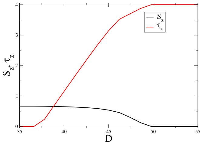
FIG. 6: Order parameters at B_{\perp} = 6\text{T} for PS1 with purely perpendicular field. Recall that D is in arbitrary units. For D < 36 , the system is in the CAF phase. It makes a second-order transition to the \text{BU}(1)^2 phase at D = 36 and remains in this phase till D = 46 , at which point it makes another second-order transition into the SVE phase. The SVE phase persists till about D = 50 , beyond which the system is fully layer polarized.
