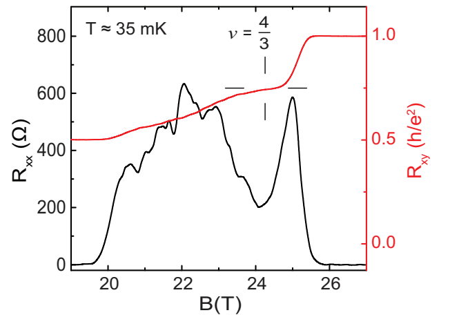
FIG. 2. R_{xx} and R_{xy} traces are shown near \nu = 4/3 . The vertical lines mark the expected magnetic field position for \nu = 4/3 . The horizontal lines indicate the expected corresponding R_{xy} quantized value ( 3h/4e^2 ).
