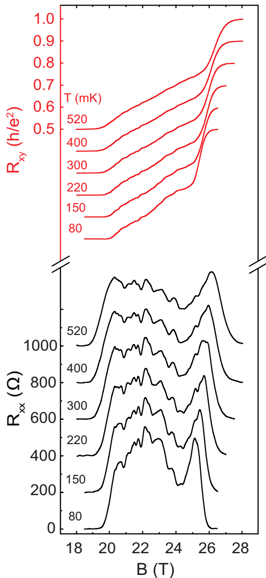
FIG. 3. Temperature dependence for the R_{xx} and R_{xy} traces between \nu = 1 and \nu = 2 . For clarity, starting from the 80 mK trace, each R_{xx} trace is shifted up vertically by 0.2 k \Omega . Similarly, each R_{xy} trace is shifted vertically by 0.1(h/e^2) as well.
