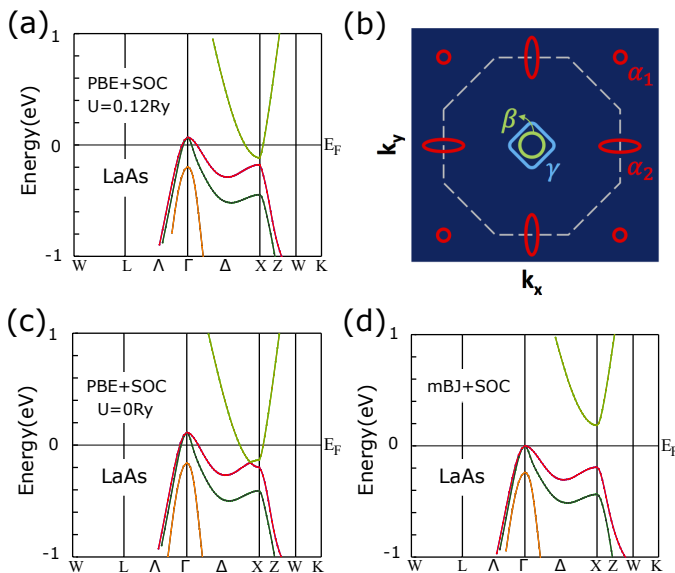
FIG. 3. (a) The correct band structure of LaAs (consistent with ARPES and quantum oscillations) from a PBE+SOC+U calculation with U = 0.12 Ry. (b) Schematic 2D map of the Brillouin zone with ellipsoidal electron pockets ( \alpha ) at the X points and concentric hole pockets (inner \beta and outer \gamma ) at the \Gamma point. (c) Band structure of LaAs calculated by PBE+SOC showing a band crossing near X. (d) Band structure of LaAs calculated by mBJ+SOC showing a large gap that lifts the electron pocket from E_F .
