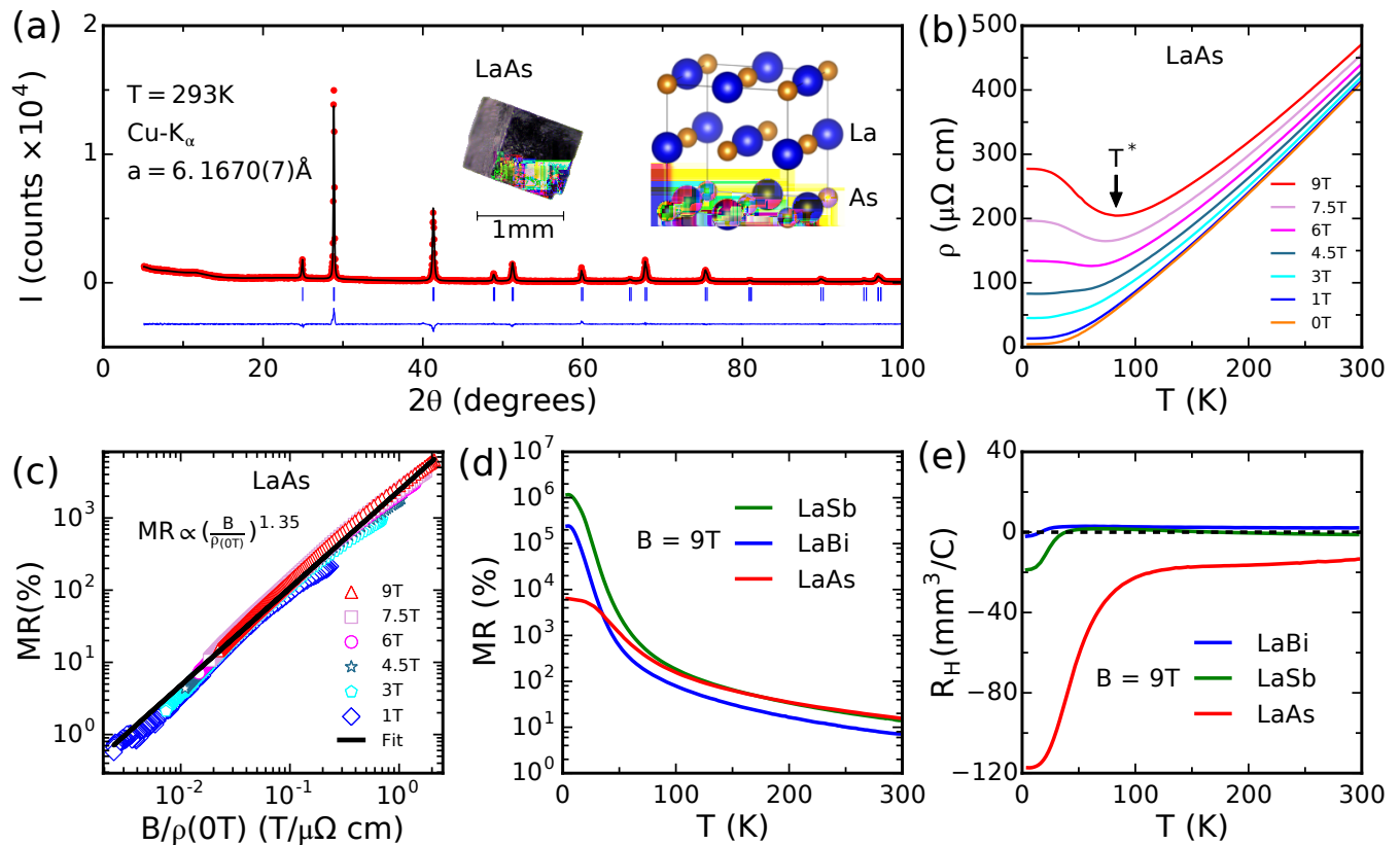
FIG. 1. (a) Rietveld refinement on the powder x-ray data from LaAs in the space group Fm\bar{3}m with R_{wp} = 7.71 , R_{exp} = 6.05 , and \chi^2 = 1.63 . Inset shows a picture of the single crystal and a drawing of the LaAs unit cell. (b) Resistivity as a function of temperature at different fields in LaAs. (c) Kohler scaling analysis on the resistivity data. (d) Magnetoresistance as a function of temperature in LaAs, LaSb, and LaBi on a logarithmic scale. (e) Hall coefficient as a function of temperature in LaAs, LaSb, and LaBi.
