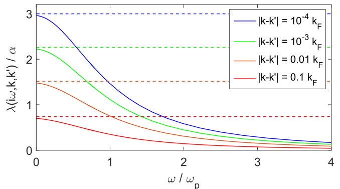
FIG. 3. The attractive part (20) of the interaction (18) normalized by \alpha vs. frequency in units of the plasma frequency, for different values of |k - k'| near the Fermi energy and for the parameters in Table I. The dashed lines represent the instantaneous repulsive part (19) for comparison and follow the same color coding.
