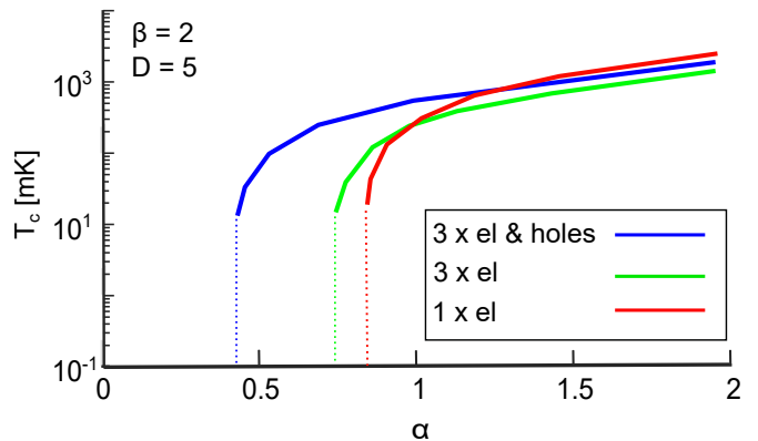
FIG. 7. The transition temperature T_c vs. the fine structure coupling constant, \alpha for three different cases: (i) with three electron pockets ( N = 3 ) and the hole pocket, (ii) only the three electron pockets and (iii) just a single electron pocket ( N = 1 ).
