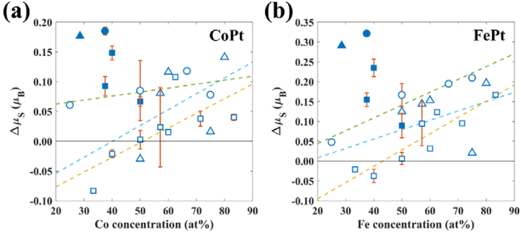
Figure 3. Predicted magnetic moment change ( \Delta\mu_S , relative to the corresponding values in bulk crystal) of the surface Pt (open symbols), Co (filled symbols), and Fe atoms (filled symbols) in the (a) CoPt and (b) FePt nanoparticles as plotted against their local chemical composition. In this figure, the triangles, squares, and circles represent the data for the CO, Dh, and Ih nanoparticles, respectively. The dashed lines are used to guide the eyes for the magnetic moment changes of the surface Pt atoms in the Ih (green), CO (cyan), and Dh (orange) nanoparticles.
