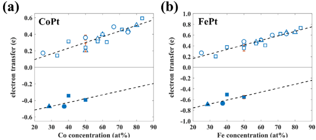
Figure 2. Predicted variation of the electron gain on the 5d Pt atoms (open symbols) as well as the electron loss on the 3d Co and Fe atoms (filled symbols) in the surface of (a) CoPt and (b) FePt nanoparticles as a function of their local chemical composition. In this figure, the triangles, squares, and circles represent the data for the CO, Dh, and Ih nanoparticles, respectively. The dashed lines are linear fitting of the data.
