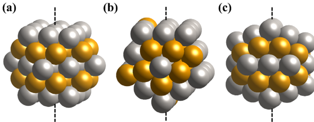
Figure 1. Atomistic structures of (a) cuboctahedral, (b) decahedral and (c) icosahedral nanoparticles. In the figure, the gray balls represent Pt atoms and the golden balls represent Co or Fe atoms. The dashed line indicates a four-fold axis of a cuboctahedral particle, a two-fold axis of a decahedral particle, and a two-fold axis of an icosahedral particle.
