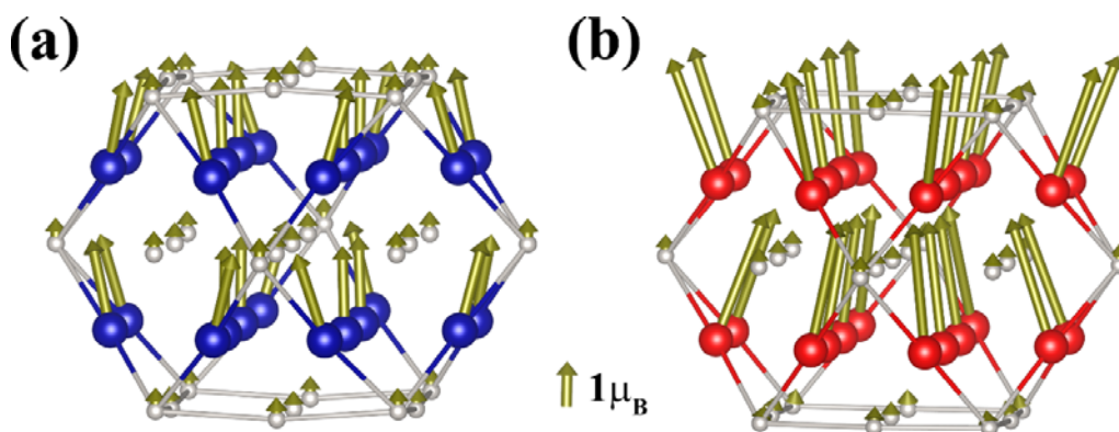
Figure 4. Surface magnetic configuration of the 55-atom cuboctahedral (a) CoPt and (b) FePt nanoparticle under vertically upward (i.e., [001] direction) magnetization predicted by the noncollinear magnetism DFT calculations. In the figure, the blue balls represent Co atoms, the gray balls represent Pt atoms, the red balls represent Fe atoms, and the golden arrows represent the atomic
