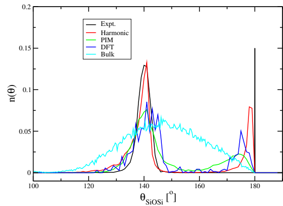
FIG. 3. The Si-O-Si bond angle distributions determined from the original experimental configuration and from the bilayers obtained using models of increasing complexity as well as for the bulk glass. The peak at \theta_{\text{SiOSi}} \sim 145^\circ arises from the “in-plane” tetrahedral links whilst the peak at \sim 180^\circ arises from the central bridging oxygen atoms between the two planes. The unrefined experimental result for the Cornell h sample is shown in black where it was assumed that the central bridging angle was exactly 180^\circ . The DFT calculation is on a computer-generated periodic sample and acts as the best guide for what to expect. The other two results are for the refined Cornell h sample using both the harmonic model and the polarizable-ion model as described in the text. Both show significant tilting as expected from the results of DFT, while maintaining the central symmetry plane.
