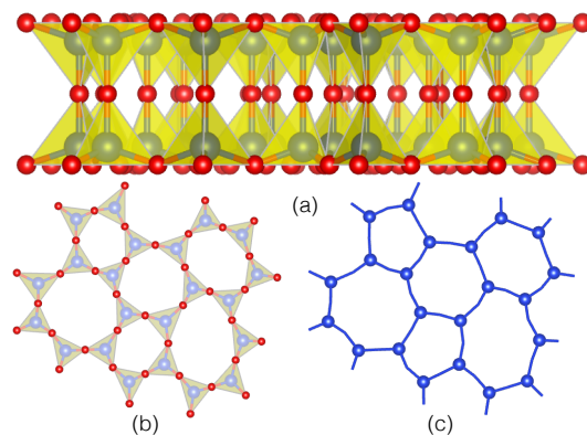
FIG. 1. (a) A small piece of silica bilayer in which oxygen atoms (red) form a tetrahedral network while silicons (blue) are located at the center of tetrahedra. (b) The top view of the silica bilayer where O and Si atoms are projected into the plane, with O forming a network of corner-sharing triangles. (c) An alternative view where Si atoms form a network of edge-sharing polygons (rings), while oxygens are removed for clarity. This view is stressed in Fig. 2.
