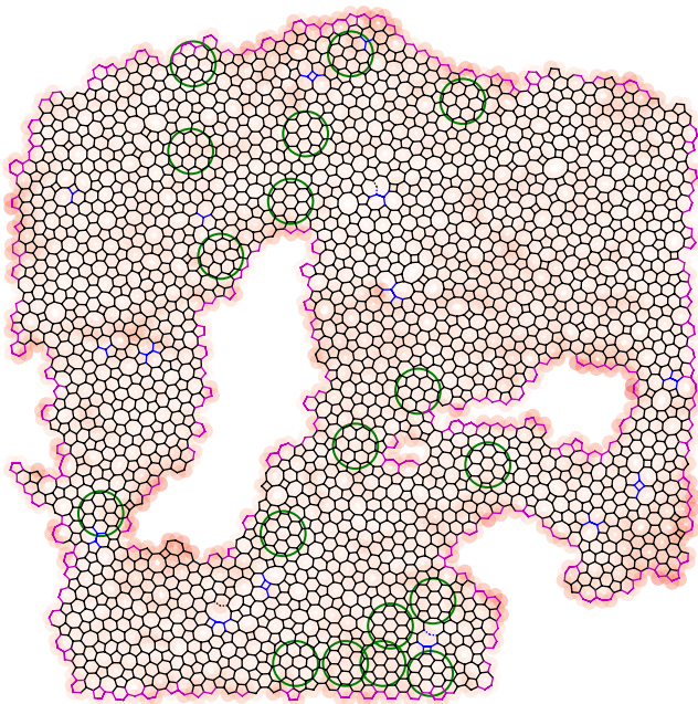
FIG. 2. The Cornell h network viewed perpendicular to the plane containing the bilayer with the O atoms removed for clarity, and only the top layer of Si atoms shown as vertices . The atoms associated with the blue and magenta bonds were not directly imaged but have been added in the computer refinement. The blue and magenta bonds highlight bonds reconstructed within the main body of the sample and at the surface, respectively. Dashed lines highlight small sections in which an under-coordinated Si atom was required for filling. The intensity of the red highlights the difference between the configuration relaxed with the spring and PIM potentials. The green circles show small crystallites .
