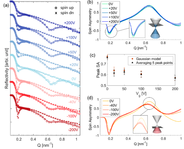
Fig. 2 (color). (a) The experimental measured (o and x dots) and theoretically refined (solid lines) PNR reflectivity (in log scale) vs. Q of both spin components R_{\uparrow} and R_{\downarrow} , at various backgate voltages V_g = 0\text{V}, +20\text{V}, +50\text{V}, +100\text{V}, +200\text{V}, -200\text{V}, -100\text{V} and -40\text{V} (based on the measuring sequence). Q is the magnitude of the neutron momentum change, where at low Q , R_{\uparrow} = R_{\downarrow} = 1 . Each reflectivity curve is vertically shifted by 10^2 for clarity. (b, d) The spin asymmetry (SA) at positive and negative V_g s, respectively. Even before any refinement, a higher spin asymmetry peak can be seen at low V_g , indicating a greater change of local magnetic structure at small V_g , as shown in (c).
