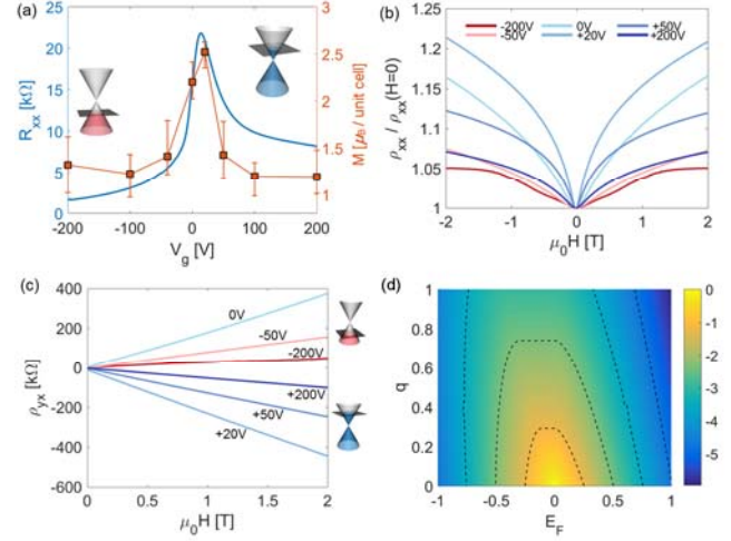
Fig. 4 (color). (a) The sheet longitudinal resistance R_{xx} of the MI/TI heterostructure (blue curve) vs the proximity induced magnetization M (orange dots), as a function of gate voltage V_g . The proximity induced magnetism shows a peak near the Dirac point, where the R_{xx} also shows a peak. (b) Normalized longitudinal magnetoresistance R_{xx}(H) , from which a typical WAL behavior is seen in almost all bias voltages. (c) Hall resistance R_{yx}(H) as a function of V_g . From the sign we could tell that at V_g = 0 V it is hole-doped ( R_{yx} > 0 ), while at V_g = 20 V it is electron-doped ( R_{yx} < 0 ). (d) The computed susceptibility \chi as a function of Fermi level E_F and wavenumber q . A diamagnetic effect \chi < 0 is shown on both sides away from the Fermi level.
