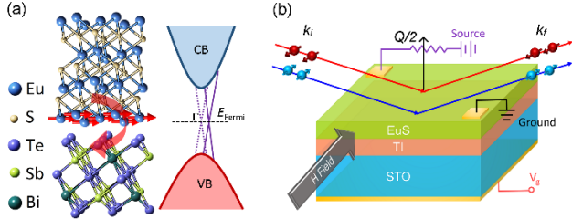
Fig. 1 (color). (a) The atomic configuration (left) and schematic band structure (right) at the MI/TI interface. When the ferromagnetic Eu ions magnetize the surface state of the TI (red arrow in left figure), the original Dirac cone (purple dotted lines) is shifted away from \Gamma point (purple solid lines) through exchange coupling, causing MPE. (b) The schematics of the gate-dependent neutron reflectometry system, where the incident neutron momentum, reflected neutron momentum and the momentum change are denoted as k_i , k_r , and (\Delta k) , respectively. The two neutron spins switched by a spin flipper shine onto the sample alternatively. See Supplemental Material I at [URL will be inserted by publisher] for an image of the setup.
