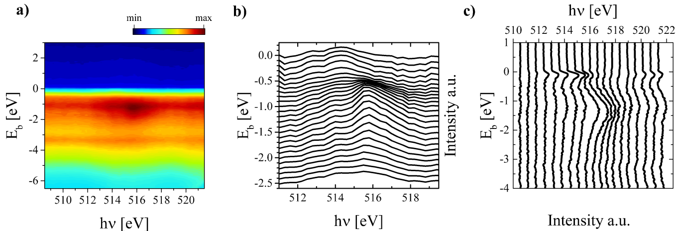
FIG. 6: a) Raw AIPES of the V_{0.06} sample as a function of h\nu across the L_3 -edge of V. b) Angular integrated constant binding energy cuts. c) The difference between AIPES measured at h\nu and off resonance (i.e. at 510 eV).
