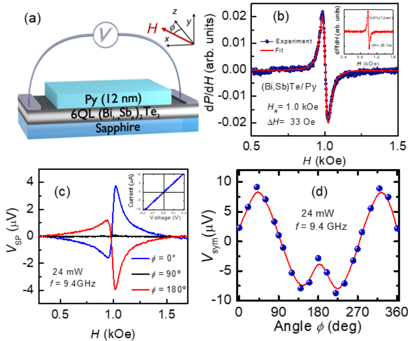
Figure 1. (color online) (a) Sketch of the bilayer sample 6QL (\text{Bi}_{0.22}\text{Sb}_{0.78})_2\text{Te}_3/\text{Py}(12\text{ nm}) and coordinate system, where \phi is the in-plane angle. (b) FMR absorption derivative versus magnetic field H measured at 9.4 GHz and microwave power of 24 mW. Inset shows the FMR spectrum for a single Py (12 nm) layer on a Si substrate. (c) Voltage measured between the electrodes for three angles of the in-plane field, with the same microwave frequency and power as in (b). Inset shows the I - V curve of the (\text{Bi}_{0.22}\text{Sb}_{0.78})_2\text{Te}_3/\text{Py} structure demonstrating the formation of Ohmic contacts between the electrodes. (d) Angular dependence of the symmetric (peak) component of the voltage line. The experimental data are represented by the solid circle symbols and the theoretical fit by the solid curve.
