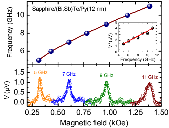
Figure 3. (color online) Lower panel: the voltage measured between the electrodes on the TI strip at the field angle \phi = 0^\circ for several microwave driving frequencies as indicated, and power 28 mW. Upper panel: Driving frequency versus the field value for the peak voltage. Inset shows the variation with frequency of the peak voltage normalized by the FMR linewidth squared referred to the value at 5 GHz.
