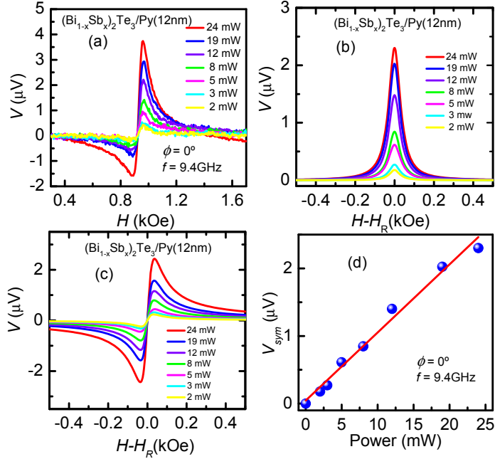
Figure 2. (color online) (a) Voltage measured between the electrodes at the field angle \phi = 0^\circ for several microwave power levels as indicated. (b) and (c) Variation with power of the symmetric and antisymmetric components of the voltage obtained by the fitting of Lorentzian and Lorentzian derivative functions to the lineshapes in (a). (d) Power dependence of the measured symmetric peak component of the voltage at \phi = 0^\circ .
