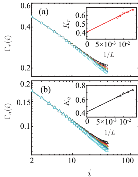
FIG. 7: The log-log plot of the single-particle density matrices \Gamma_{q,r}(i) versus the distance i for the MCJC model at the integer filling N/L = 1 with g_{l,r}/2\pi = 150 MHz. Insets: the Luttinger parameters K_{q,r} versus 1/L . The curves are for L = 80, 90, 100, 110, 120 from top to bottom.
