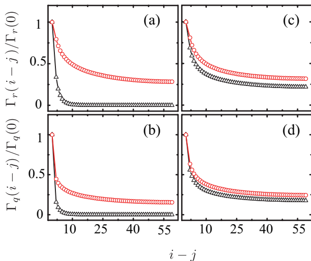
FIG. 4: The normalized single-particle density matrices \Gamma_r(i-j)/\Gamma_r(0) and \Gamma_q(i-j)/\Gamma_q(0) versus (i-j) for the MCJC model with L = 120 at integer (a,b) and half (c,d) filling. Circles: g_{l,r}/2\pi = 150 MHz; triangles: g_l/2\pi = 55 MHz, g_r/2\pi = 245 MHz.
