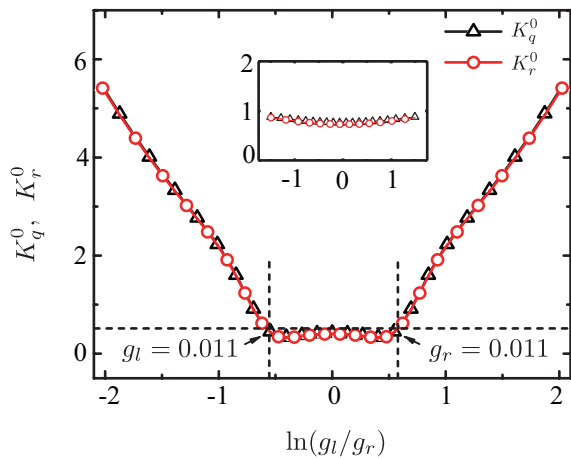
FIG. 8: The Luttinger parameters K_q^0 and K_r^0 versus \ln(g_l/g_r) at N/L = 1 with (g_r + g_l)/2\pi = 300 MHz. The dashed horizontal line is K_\alpha^0 = 1/2 . Inset: K_{q,r}^0 at N/L = 1/2 .
