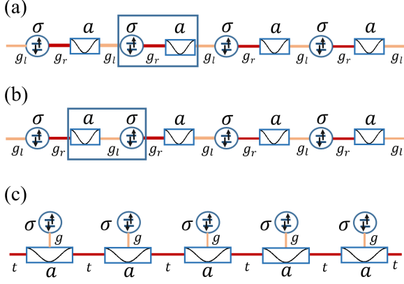
FIG. 1: The schematic of a 1D MCJC (a, b) and a CCA (c). The circles represent the qubits and the blocks represent the cavities. A unit cell of the MCJC consists of a qubit and an adjacent cavity coupled to the qubit via (a) g_r or (b) g_l .
