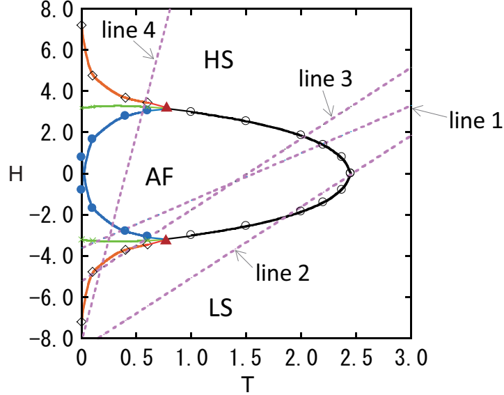
FIG. 1: (color online) (a) Phase diagram for the weak interaction case of the elastic model. The black line denotes the critical line. Orange and blue lines are spinodal lines for AF-like and F-like phases, respectively. Green lines denote the coexistence lines of the AF-like and F-like (HS or LS) phases. Red triangles are tricritical points. Lines 1-4 (four dashed lines) are paths for typical SC transition patterns (see Fig. 2).
