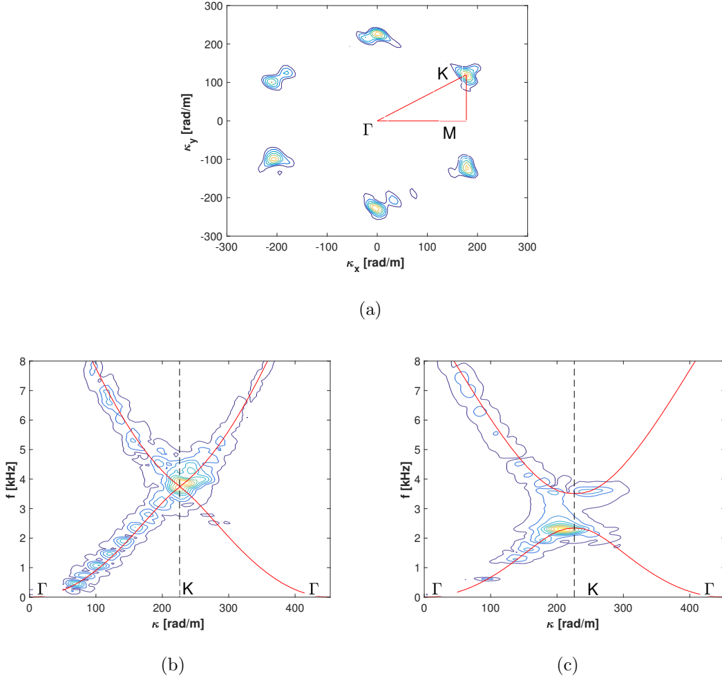
FIG. 5: Experimental 3D-FTs. Lattice with \gamma = 0 : cross section |\hat{w}(\kappa_x, \kappa_y, \omega)| at frequency f_0 \approx 3.75 kHz close to the numerically predicted Dirac cone (a). Frequency/wavenumber representation |\hat{w}(\kappa|_{\mathcal{C}}, \omega)| along the path \mathcal{C} : \Gamma - K - \Gamma and comparison with COMSOL predictions (solid red line): lattice with \gamma = 0 (b), and \gamma = 1 (c).
