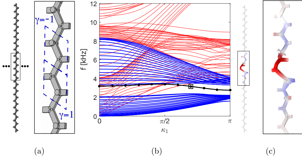
FIG. 4: Finite strip and close-up of the topological interface (a). Dispersion diagram: edge mode (dotted black line), out-of-plane modes (thick blue lines), and in-plane polarized modes (thin red lines) (b). Eigenvector corresponding to the edge mode evaluated for wavenumber \kappa_x = 0.7\pi at f \simeq 3 kHz (c).
