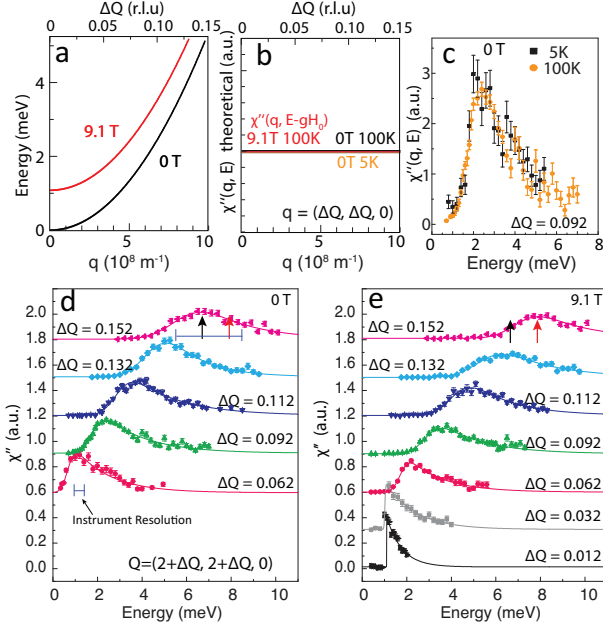
FIG. 2: (a) Schematic illustration of the expected magnon dispersions at 0 T and 9.1 T for a simple ferromagnet. (b) The expected temperature, magnetic field dependence of low-energy \chi''(\mathbf{Q}, E) for simple ferromagnet obtained from SpinW software package [39]. Here the magnetic field induced spin gap gH_0 has been subtracted in the 9.1 T \chi''(q, E - gH_0) (red). The upper and bottom units are \Delta Q and q , respectively. (c) Our estimated \chi''(\mathbf{Q}, E) with \mathbf{Q} = (2.092, 2.092, 0) at 5 K and 100 K after correcting measured S(\mathbf{Q}, E) for the background and Bose-population factor. (d,e) The estimated \chi''(\mathbf{Q}, E) at 0 T and 9.1 T, respectively, after correcting for background and Bose population factor. Scans at different wave vectors are lifted up by 0.3 sequentially. The black and red arrows marks the peak positions at 0 T and 9.1 T, respectively.
