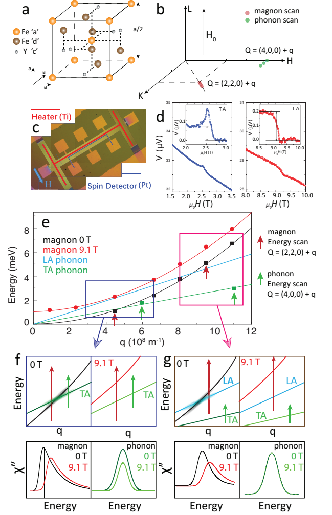
FIG. 1: (a) The full unit cell of YIG comprises eight cubes that are related by glide planes to the basic cube shown in the figure. (b) The corresponding reciprocal space with the [H, K, 0] scattering and vertical magnetic field H_0 . The red and green solid circles mark the positions of reciprocal space where we probe spin waves and acoustic phonons, respectively. (c) A picture of the Pt/YIG device used for SSE measurements. (d) SSE voltage in the field ranges where anomalous features appear at 100 K. (e) Magnon and phonon dispersions of YIG at 100 K and different magnetic fields. The black squares and solid red circles are data from 0 T and 9.1 T measurements, respectively. The q \approx 4.5 \times 10^8 \text{ m}^{-1} point corresponds to \Delta Q = 0.062 in Fig. 2(d). The black and red solid lines are quadratic ferromagnetic spin wave fit to the data. The blue and red boxes indicate magnon-phonon crossing points. The green and blue solid lines are TA (with phonon velocity C_{\perp} \approx 3.9 \times 10^3 \text{ m/s} ) and LA ( C_{\parallel} \approx 7.2 \times 10^3 \text{ m/s} ) phonons, respectively [31]. (f, g) The expanded view of the blue and red boxes in (e), respectively. The bottom panels in (f, g) summarize the results obtained in our measurements on the magnetic field effect on spin waves, hybridized excitations, and TA phonons.
