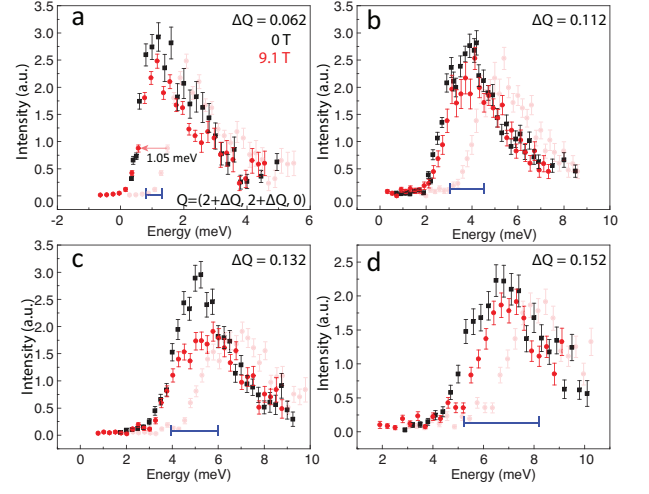
FIG. 3: (a,b,c,d) Comparison of the estimated \chi''(\mathbf{Q}, E) as a function of increasing wave vector at 0 T (black) and 9.1 T (red). The 9.1T data is shifted by 1.05 meV to accommodate the field induced energy shift. Light red dots represents the original data position of the 9.1 T data. The horizontal bars are estimated instrumental energy resolution based on magnon dispersion at 100 K.
