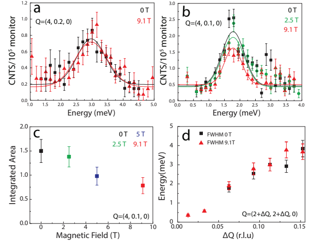
FIG. 4: (a) Energy scan of S(\mathbf{Q}, E) at \mathbf{Q} = (4, 0.2, 0) , a position far away from magnon-phonon crossing points, and 100 K to probe TA phonon at 0 T and 9.1 T (b) Energy scan of S(\mathbf{Q}, E) to probe magnon-phonon hybridized excitations at \mathbf{Q} = (4, 0.1, 0) near magnon-phonon crossing point at 0 T, 2.5 T, and 9.1 T. (c) Magnetic field dependence of the integrated intensity of magnon-phonon hybridized excitations at 100 K and \mathbf{Q} = (4, 0.1, 0) . (d) FWHM of the magnon at 0 T and 9.1 T as a function of \Delta Q .
