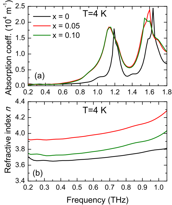
FIG. 3: (Color online) THz absorption (a) and refractive index (b) of \text{CaBaCo}_4\text{O}_7 pellets with different Ni content.
