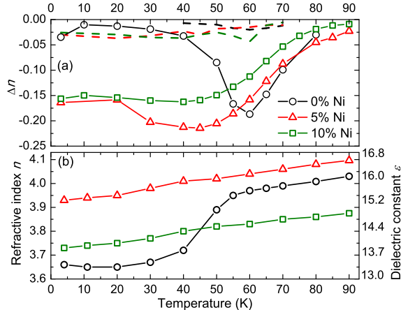
FIG. 5: (Color online) (a) Solid lines with symbols plot the magnetic field induced change in refractive index \Delta n(\omega) = n(\omega, B) - n(\omega, 0 \text{ T}) at frequency \omega = 0.4 THz and in applied field B = 17 T. Dashed lines plot the quantity \Delta n_1(\omega) , Eq. (6). (b) Temperature dependence of refractive index n(\omega) at frequency \omega = 0.4 THz and in zero magnetic field. The vertical axis on the right hand side indicates the real part of the dielectric function at 0.4 THz calculated from n(\omega) = \sqrt{\epsilon_1(\omega)} .
