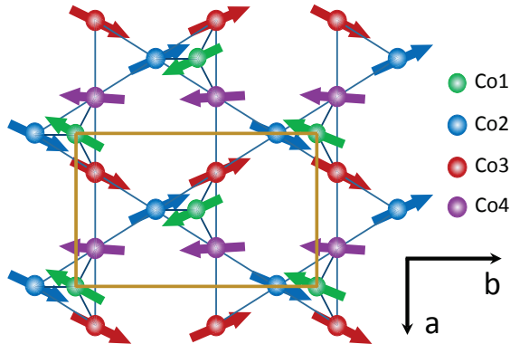
FIG. 1: (Color online) Magnetic structure of CaBaCo 4 O 7 . Triangular layers are formed by the Co1 ions. Kagome layers are formed by Co2, Co3, and Co4 ions.
