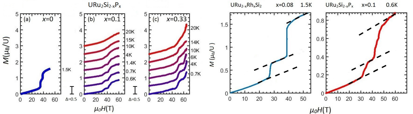
FIG. 5: Magnetization versus magnetic field \mu_0H for Rh-substituted [24] and P-substituted URu_2Si_2 at low temperatures in the no-order x -regime. Dashed lines are guides to the eye to illustrate the 1/3 and 2/3 magnetization jumps seen in each material.
