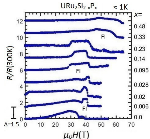
FIG. 2: Waterfall plot of normalized electrical resistance R/R(300\text{K}) vs. magnetic field \mu_0 H for various concentrations of x at T \approx 1 K. Each trace is offset by an amount \Delta = 1.5 . The field induced FI phase originates as a narrow region in field in the HO x -regime ( 0 < x < 0.035 ) and expands to a much broader range in the no-ordered x -regime ( 0.035 < x < 0.26 ). The FI order may persist at high fields in the AFM x -regime ( 0.26 < x < 0.5 ).
