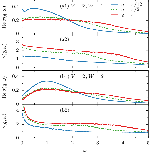
Figure 3. (Color online) (a1,b1) \text{Re } \sigma(q, \omega) and (a2,b2) \gamma(q, \omega) (MCLM, L = 24 ) for fixed V = 2 , few different q , and two disorders: (a) W = 1 and (b) W = 2 .
