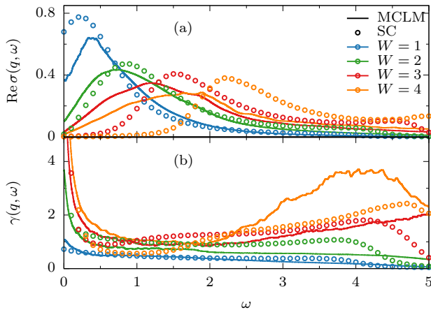
Figure 4. (Color online) Comparison between SC and numerical (MCLM) results of (a) \text{Re } \sigma(q, \omega) and (b) \gamma(q, \omega) for q = \pi/12 , L = L^* = 24 , and various disorder strengths W = 1, 2, 3, 4 .
