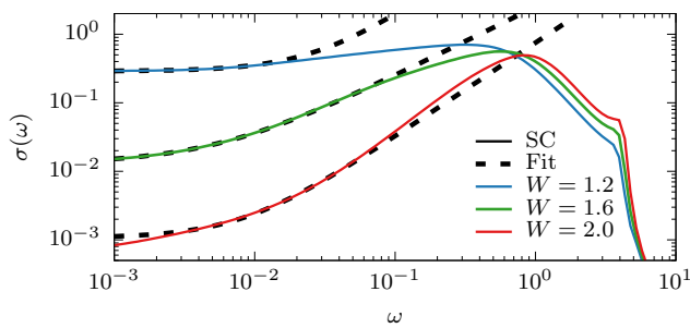
Figure 5. (Color online) Comparison of SC solution (solid line, L^* = 40 , \delta\omega = 10^{-3} ) with the fit \tilde{\sigma}(\omega) = a + b|\omega|^c (dashed line). with c = 0.8, 1.0, 1.5 for W = 1.2, 1.6, 2.0 , respectively.
