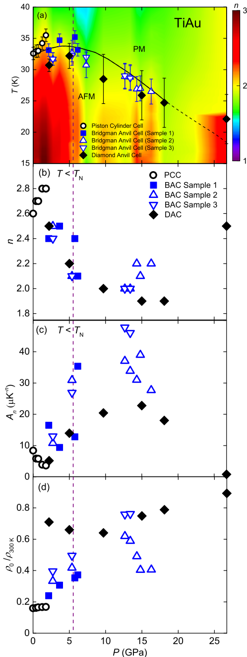
FIG. 5. (Color online) (a) Temperature vs pressure ( T_N vs P ) phase diagram superimposed on a color contour representation of the exponent n(P, T) from the electrical resistivity: \rho = \rho_0 + A_n T^n (see text). The solid black curve is a guide to the eye and denotes the T_N(P) phase boundary. (b, c, d) The parameters n , A_n , and \rho_0 vs pressure P were extracted from power law fits of the electrical resistivity in the AFM phase as shown in Fig. 4. The dashed vertical line at P = 5.5 GPa is a guide to the crossover at the peak in T_N(P) .
