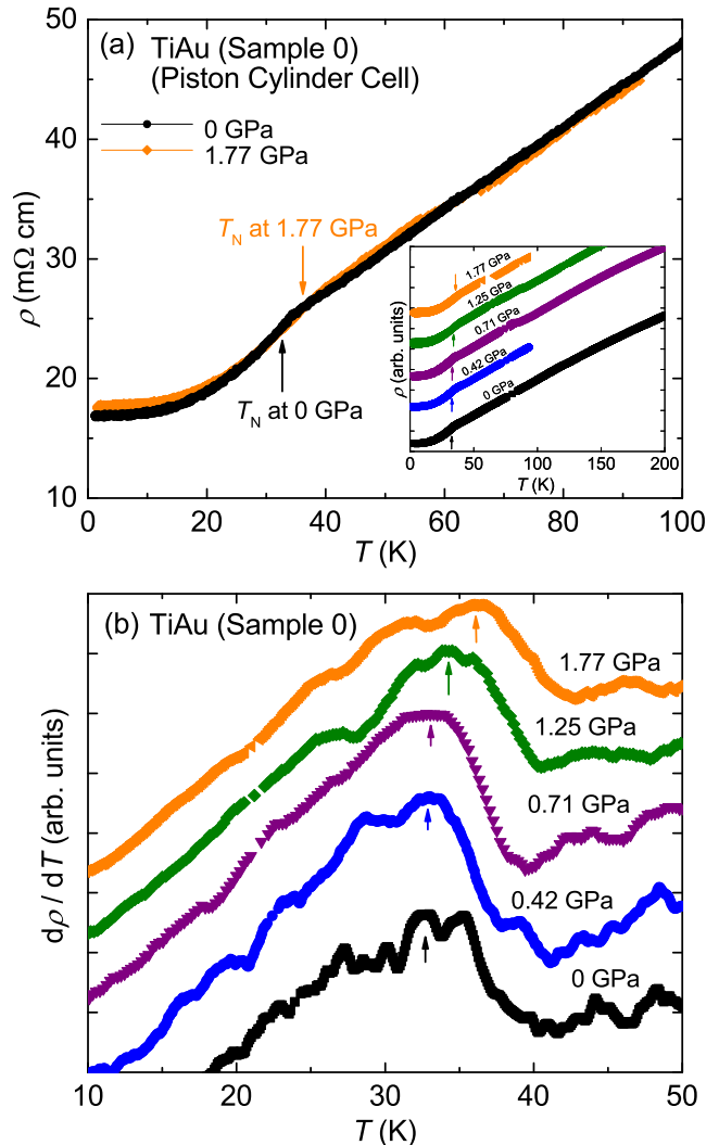
FIG. 1. (Color online) (a) Electrical resistivity \rho vs temperature T at P = 0 and 1.8 GPa as measured in a piston cylinder cell (PCC). The arrows indicate the features in \rho that correspond to values of T_N = 32.7 K and 35.5 K at P = 0 and 1.77 GPa, respectively. Inset: Electrical resistivity \rho vs T up to T = 200 K at various pressures up to P = 1.8 GPa displaying the nearly linear temperature dependence and metallic behavior of \rho in the PM phase. The \rho vs T curves have been shifted vertically for clarity in illustrating the increase in T_N with increasing pressure. (b) The temperature derivative of the electrical resistivity d\rho/dT vs temperature T at various pressures (shifted vertically for clarity). The Néel temperature at each pressure was determined from the maximum in d\rho/dT as indicated by the arrows and the values of T_N are listed in Table I.
