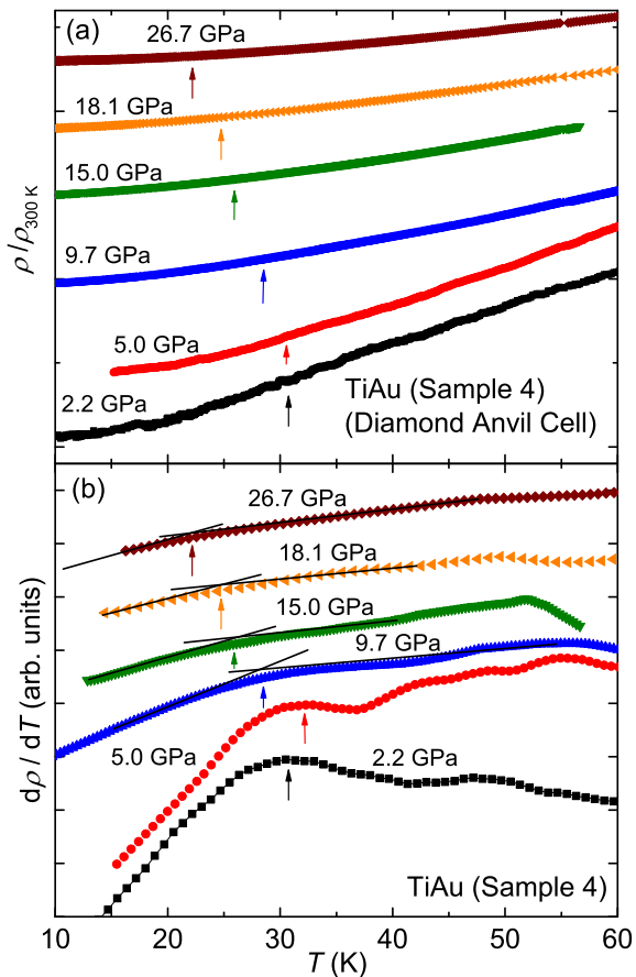
FIG. 3. (Color online) (a) Electrical resistivity \rho/\rho_{300\text{K}} vs temperature T in the vicinity of the AFM ordering temperature T_N at various pressures up to P \sim 27 GPa as measured in a diamond anvil cell (DAC). The arrows point to the features at T_N . (b) Temperature derivative of the electrical resistivity d\rho/dT vs T . The values of T_N = 30.7 and 32.2 K at P = 2.2 and 5.0 GPa respectively were determined from the maximum in the d\rho/dT vs T curves whereas the values of T_N = 28.5, 25.9, 24.7, 22.1 K at P = 9.7, 15.0, 18.1, 26.7 GPa, respectively, were determined from the intersection of the linear extrapolations (solid black lines) of the d\rho/dT vs T curves as shown in panel (b).
