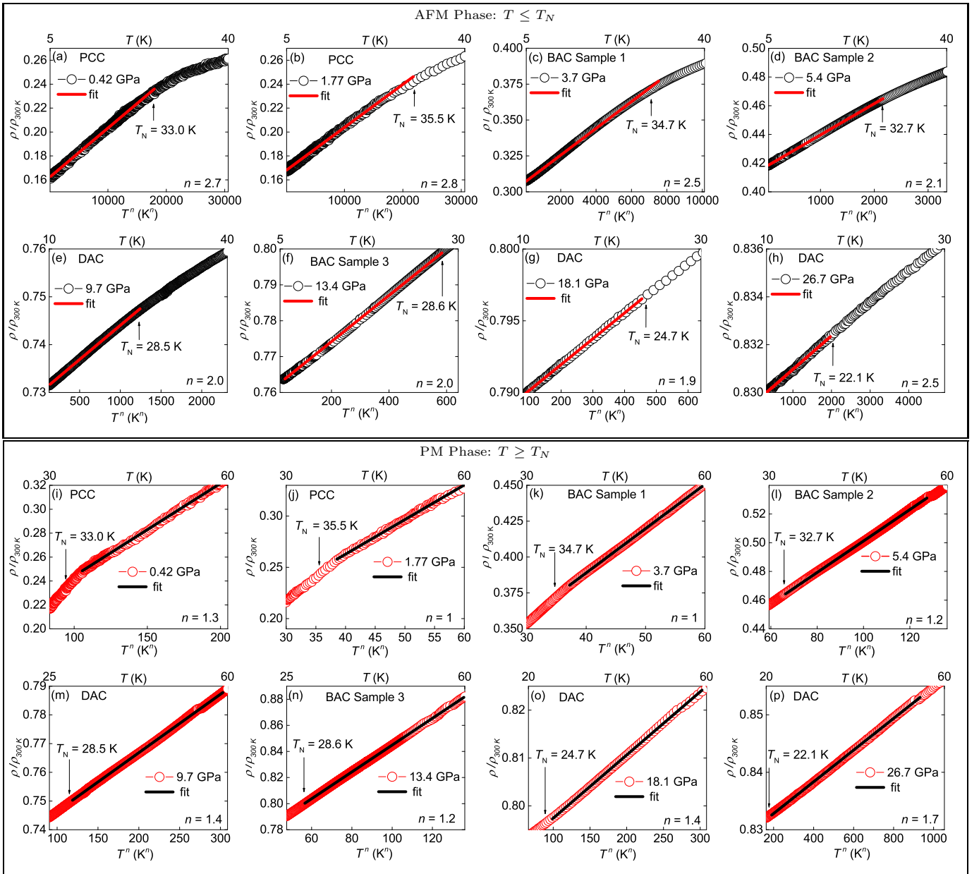
FIG. 4. (Color online) Scaled electrical resistivity \rho/\rho_{300\text{K}} vs T^n above and below the Néel temperature T_N for TiAu under pressure, P . Power law fits of the electrical resistivity, \rho = \rho_0 + A_n T^n to the \rho(T) data were performed for T < T_N in the AFM phase (top 8 panels with black symbols and a red fit line) and for T > T_N in the PM phase (bottom 8 panels with red symbols and a black fit line). The upper x-axis in each plot is shown as a linear T scale and T_N is indicated by the black vertical arrows.
