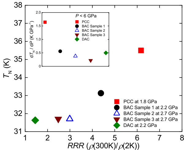
FIG. 6. (Color online) A plot of the T_N vs residual resistivity ratio RRR = \rho(300 \text{ K})/\rho(2 \text{ K}) for the five TiAu samples measured in each of the various pressure cells at a low pressure of P \sim 2 to 3 GPa. Inset: Pressure coefficient dT_N/dP during the enhancement of T_N as pressure is increased up to P \sim 6 GPa for the five different TiAu samples.
