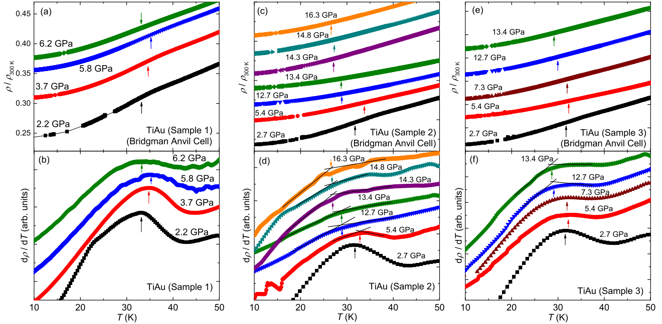
FIG. 2. (Color online) Electrical resistivity \rho/\rho_{300\text{K}} (a, c, e), and its temperature derivative d\rho/dT (b, d, f), as a function of temperature for three different polycrystalline samples of TiAu, as measured in a Bridgman anvil cell (BAC) at various values of pressure. The arrows indicate the feature at the AFM ordering temperature with the values of T_N extracted either from the maximum in d\rho/dT , or from the intersection of the linear extrapolations (solid black lines) of the d\rho/dT vs T curves. The values of T_N at various P for TiAu samples 1, 2, and 3 measured in the two different Bridgman anvil cells are presented in Table I.
