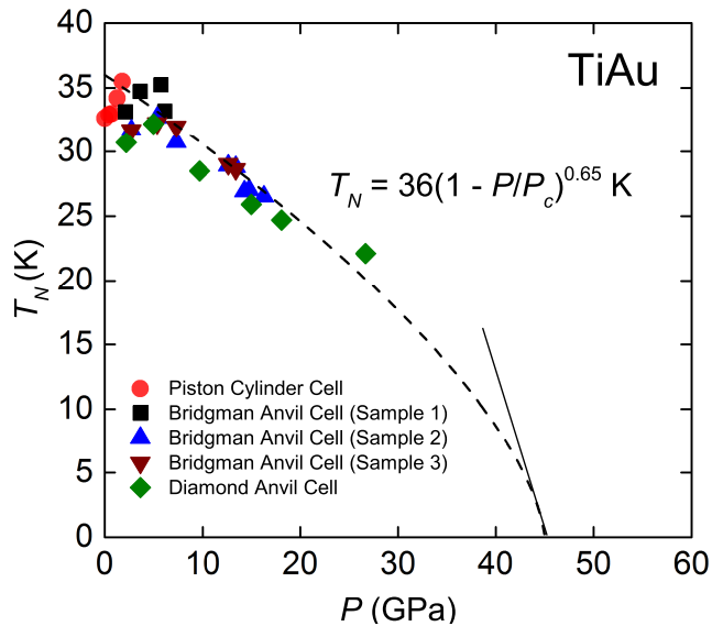
FIG. 7. (Color online) (a) A temperature vs pressure ( T_N vs P ) phase diagram for TiAu showing the extrapolated T_N(P) boundary (dashed curve) toward a critical pressure P_c at T = 0 \text{ K} . The critical scaling function T_N = T_{N(P=0)} \times (1 - P/P_c)^\alpha was fit to the T_N(P) data up to P = 27 \text{ GPa} . The ambient pressure value of the Néel temperature ( T_{N(P=0)} ) was set to 36 K while a rough estimate of the value for the critical pressure was determined from the fit to be P_c = 45 \pm 11 \text{ GPa} . The value for the scaling exponent \alpha was determined from the fit to be \alpha = 0.65 \pm 0.20 . The slope of the curve near T_N = 0 \text{ K} (represented by the solid black line) is dT_N/dP \sim -2.5 \text{ K GPa}^{-1} , while the slope of the nearly linear T_N(P) data accumulated from the various pressure cells up to P = 27 \text{ GPa} is dT_N/dP = -0.59 \text{ K GPa}^{-1} .
