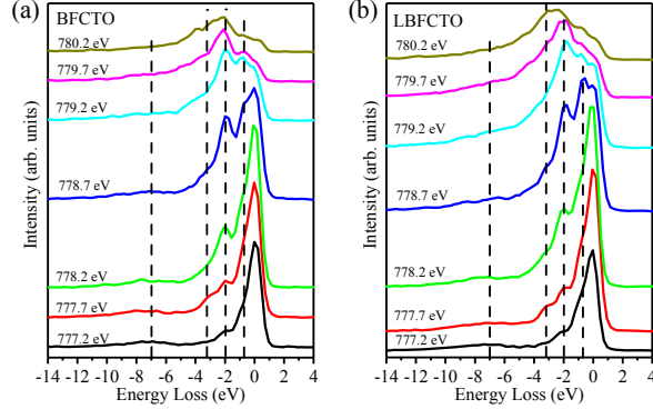
FIG. 4. Co L-edge RIXS spectra of (a) BFCTO and (b) LBFCTO films at selected incident photon energies. The incident photon energies are displayed next to the corresponding RIXS spectra and indicated by vertical sticks in Fig. 2(b).
