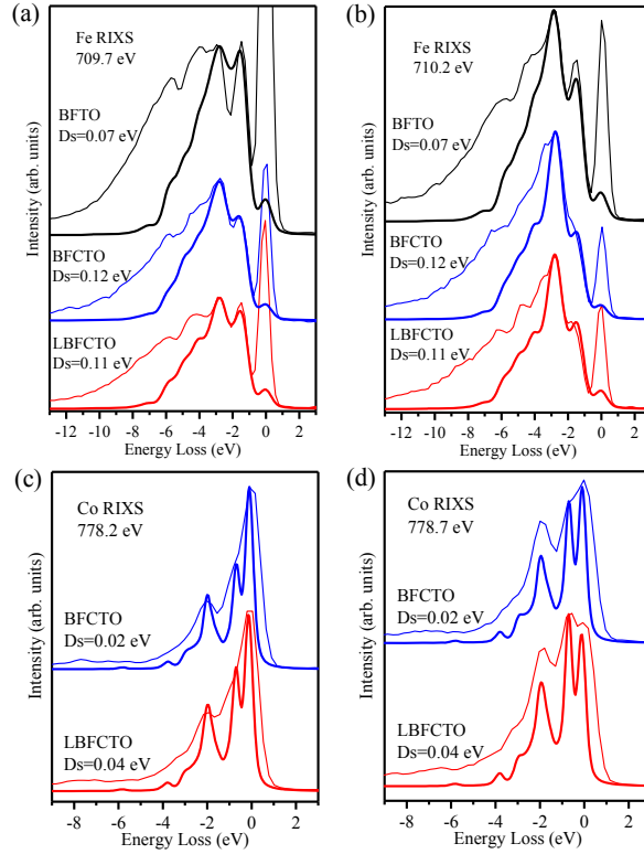
FIG. 5. Simulated \text{Fe}^{3+} (top panel) and \text{Co}^{2+} (bottom panel) L-edge RIXS spectra (thick curves) as a function of D_s in comparison with the experimental spectra (thin curves) of BFTO, BFCTO, and LBFCTO films at the incident photon energy of (a) 709.7 eV, (b) 710.2 eV, (c) 778.2 eV, and (d) 778.7 eV. The intensities of simulated spectra are all rescaled for clarity.
