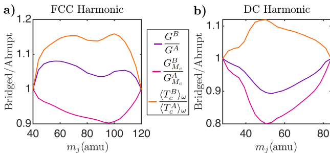
Figure 4. In the harmonic limit, the conductance of a bridged interface results from an interplay between increasing the transmission \langle T_c \rangle_\omega due to decreasing the “mismatch” at each boundary and decreasing the number of conserving modes due to a new restriction on the conservation of momentum coming from the intermediate material.
