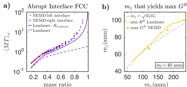
Figure 6. a) \langle MT \rangle_\omega , plotted per conventional unit cell, is a function of the mass ratio for abrupt interfaces. b) Junction mass m_j that leads to minimum resistance vs. right contact mass m_r , while keeping the left contact mass fixed. The mass follows closely the geometric mean of the contact masses.
