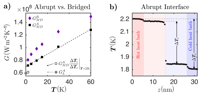
Figure 3. a) Conductance of the abrupt interface G_{MD}^A and maximum conductance of the bridged interface G_{MD}^B vs. temperature for a FCC crystal calculated from NEMD. The rapid increase of G_{MD}^B at low T highlights the important role of anharmonicity enhancing G_{MD}^B relative to G_{MD}^A . b) Temperature profile of the abrupt interface from NEMD. This profile allows us to include the contact resistances into the NEMD conductance (Eq. 2), which shows excellent agreement with our Landauer calculations G_L^A .
