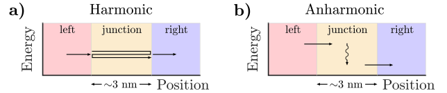
Figure 1. Interface with an added intermediate layer or junction (bridged interface) a) In the harmonic limit, the layer behaves like an impedance matcher that increases transmission by constructive interference while reducing the number of conducting modes due to energy-momentum conserving constraints. b) In the anharmonic limit, the layer behaves as a bridge for phonon down and up conversion that increases the chances of phonons crossing the interface.
