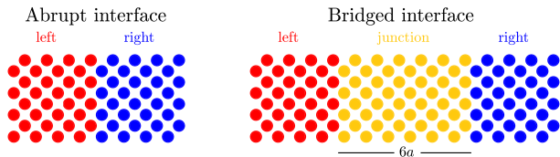
Figure 7. Lateral view of the abrupt and bridged interfaces simulated in this work. Each ball represents a primitive unit cell.
