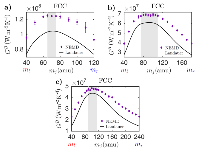
Figure 8. Conductance vs. junction mass for different right contact masses. a) m_r = 120 amu, b) m_r = 180 amu, c) m_r = 240 amu. The shaded area shows the masses whose NEMD conductance enhancement is within 5% of the maximum enhancement. The Landauer curves come from Eq. 9– R_j using \langle MT \rangle_\omega from Landauer (solid line Fig. 6b).
