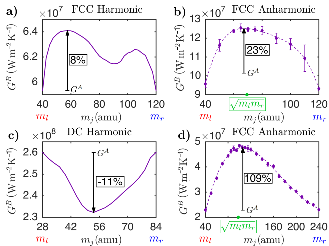
Figure 2. Conductance of bridged interfaces as the atomic mass of the intermediate layer or junction is varied between the contact masses. The conductance of the abrupt interface is indicated by the tail of the arrow. In the harmonic limit, a FCC crystal shows a relative enhancement of conductance from abrupt to bridged interface a) , while a DC crystal shows the opposite c) . In the anharmonic regime b) , the conductance enhancement of a FCC crystal is three times larger than that of the harmonic limit a) . Moreover, the maximum enhancement happens when the junction mass is close to the geometric mean of the contact masses ( c) m_r = 120 amu and d) m_r = 240 amu). The dashed lines are fourth order polynomial functions that fit the NEMD data.
