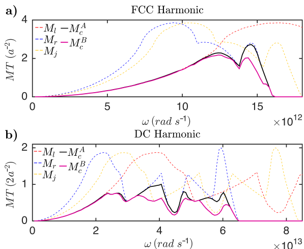
Figure 5. Available modes for the contacts and junction, and conserving modes of the bridged and abrupt interface. Adding the junction puts an extra constraint on the conserving modes that hurts M_c and decreases the number of available modes. We plot the cases in which G_{M_c} is minimum: m_j = 96 amu for FCC crystal and m_j = 50.4 amu for the DC crystal.
