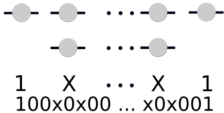
FIG. 2. Same as Fig. 1, but for the sphere, where the first excited LL has one more orbital at both maximum and minimum L_z , for both electrons and composite fermions. Shown (bottom line) is the resulting unique dominance pattern for a sphere satisfying 2s = \frac{5}{2}N - 4 , where 2s is the number of flux quanta penetrating the sphere.
