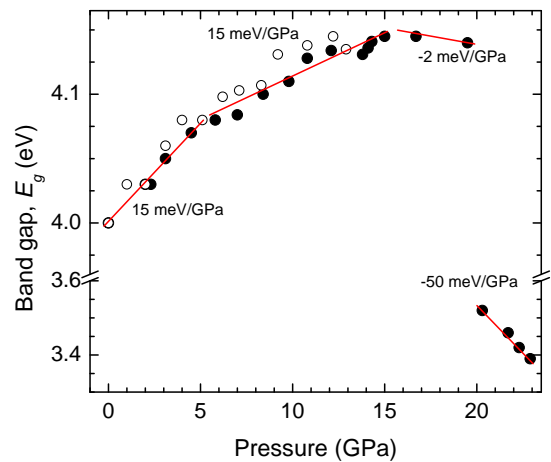
FIG. 4: Pressure dependence of the band gap energy of \text{CdWO}_4 . Open circles represent data from Ref. 10 while filled circles are from data collected in this study. The continuous red lines show the fits.
