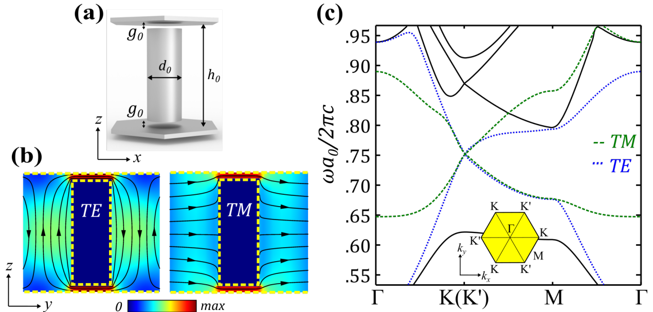
Figure 1: The unperturbed “photonic graphene” (PhG) structure used for emulating photon equivalents of the spin and valley degrees of freedom. (a) The unit cell of the PhG: metal rods arranged as a hexagonal array lattice with the lattice constant a_0 . (b) Magnetic field profiles of the TE and TM modes at the K point. (c) The PBS with TE and TM modes forming doubly-degenerate Dirac cones at K(K') points. Design parameters: h_0 = a_0 , d_0 = 0.345a_0 , and g_0 = 0.05a_0 .
