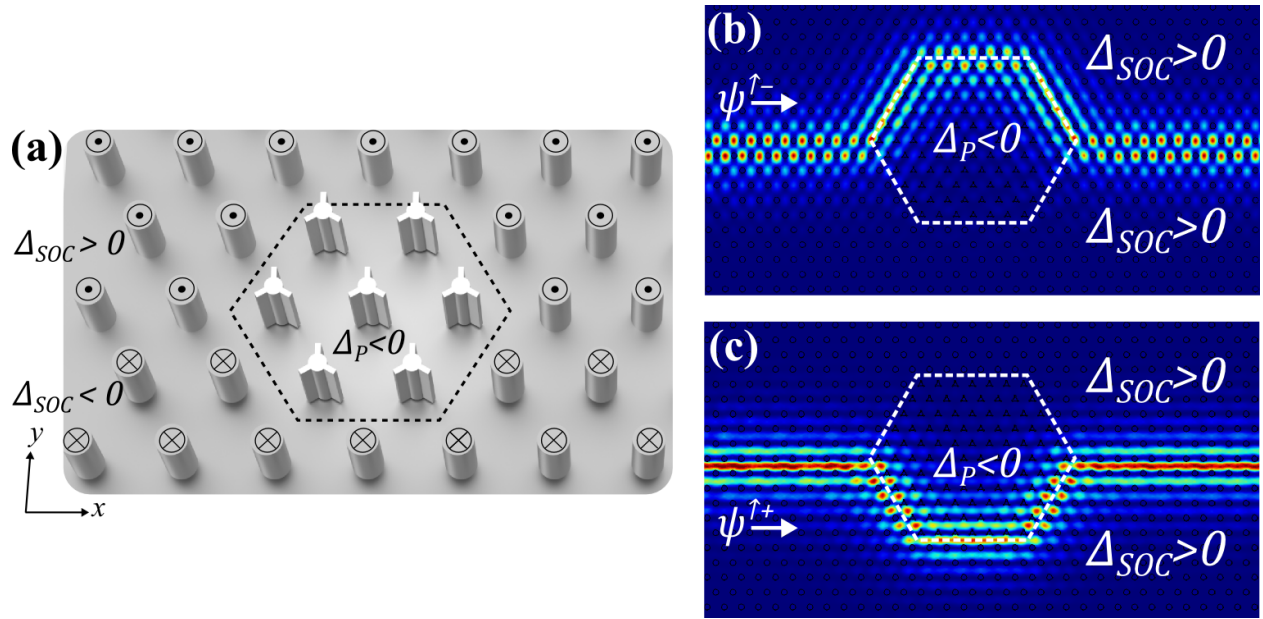
Figure 7: Valley-filtering of TPEWs. (a) Schematic: a QVH-PTI cavity with \Delta_p < 0 embedded in a QSH-PTI matrix containing an interface between \Delta_{SOC} > 0 (dots) and \Delta_{SOC} < 0 (crosses) domains. (b,c) Valley-dependent deflection of TPEWs launched into the (b) K -valley (negative index) and (c) K' -valley (positive index) modes. The K/K' -valley TPEWs are deflected to the upper/lower arms of the embedded cavity. Color: |E_z|^2 .
