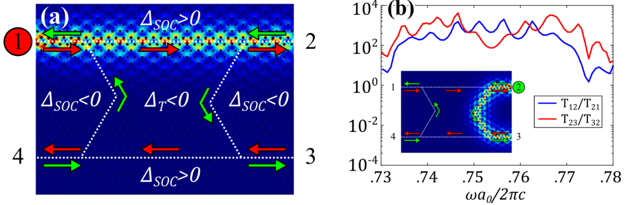
Figure 8: Four-port circulator based on (a) a QH-PTI cavity with \Delta_T < 0 embedded into a QSH-PTI matrix with two domain walls separating the \Delta_{SOC} < 0 domain from the \Delta_{SOC} > 0 domains. White dashed lines: interfaces between PTIs with indicated signs of \Delta 's. Red (green) arrows: propagation directions of TPEWs with up-spin (down-spin) supported by the interfaces. (a) Energy density profile of TPEW launched from port 1 and heading port 2. (b) The isolation ratio spectra for two different launching ports. Inset: energy density profile of TPEW launched from port 2 and heading port 3. QSH-PTIs' parameters: h_0 = a_0 , d_0 = 0.346a_0 , g_{SOC} = 0.1a_0 . QH-PTIs' parameters: h_0 = a_0 , d_0 = 0.346a_0 , g_T = 0.05a_0 , gyromagnetic material parameters are the same as Fig.2(b).
