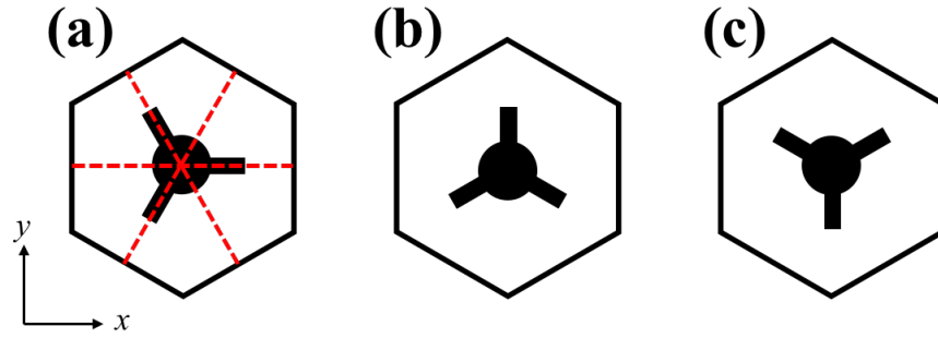
Figure 4: Three representative unit cells of QVH-PTI. (a) A unit cell with the tips of the tripod pointing along \Gamma - K(K') directions (red dashed lines) that does not break the inversion symmetry. (b,c) Tripod orientations that maximize the absolute values |\Delta_P| of the bandgap. The signs of \Delta_P are opposite for (b) and (c): \Delta_P < 0 for (b), and \Delta_P > 0 for (c).
