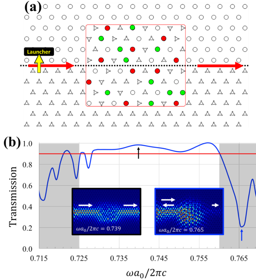
Figure 6: Topological protected edge wave against a large disordered defect. (a) A disordered defect is an 8 \times 8 array of random unit cells inside the red box. The circles represent QSH-PTI unit cells with the top plate gaps sized at g_{\text{SOC}} = 0.15a_0 (white), g_{\text{SOC}} = 0.09a_0 (green), and g_{\text{SOC}} = 0.03a_0 (red). The tripods represent QVH-PTI unit cells with different orientations. The red arrows indicate the propagation of the TPEW launched along the domain wall between QSH-PTI and QVH-PTI. (b) Transmission spectrum of the TPEW. Red line marks T = 0.9 to guide the eye.
