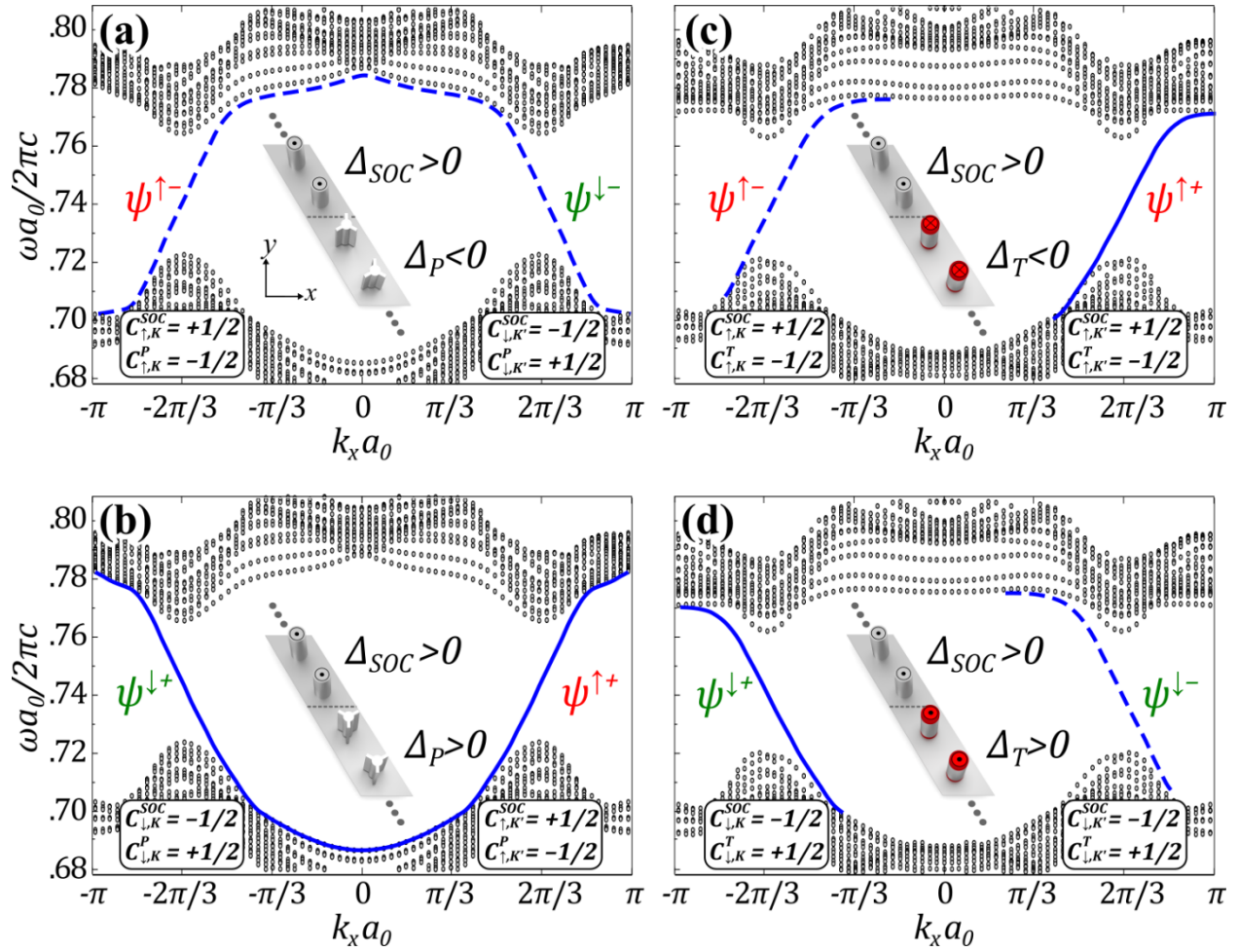
Figure 5: Topologically protected edge waves (TPEWs) propagating along zigzag-type interfaces between heterogeneous PTI claddings. Photonic band structures of the super-cells containing (a,b) QSH/QVH, and (c,d) QSH/QH PTI interfaces. The super-cells contain a single cell along the propagation x -direction and 20 cells on each side of the interface. Black circles: bulk modes, blue solid/dashed lines: dispersion curves of the TPEWs with positive/negative ( +/- ) refractive indices and \uparrow/\downarrow spins. Boxed tags: spin-Chern and valley-Chern numbers of the bulk modes below the bandgap that belong to top/bottom claddings. Due to band-folding, k_x < 0 ( k_x > 0 ) modes originate from K ( K' ) valleys.
