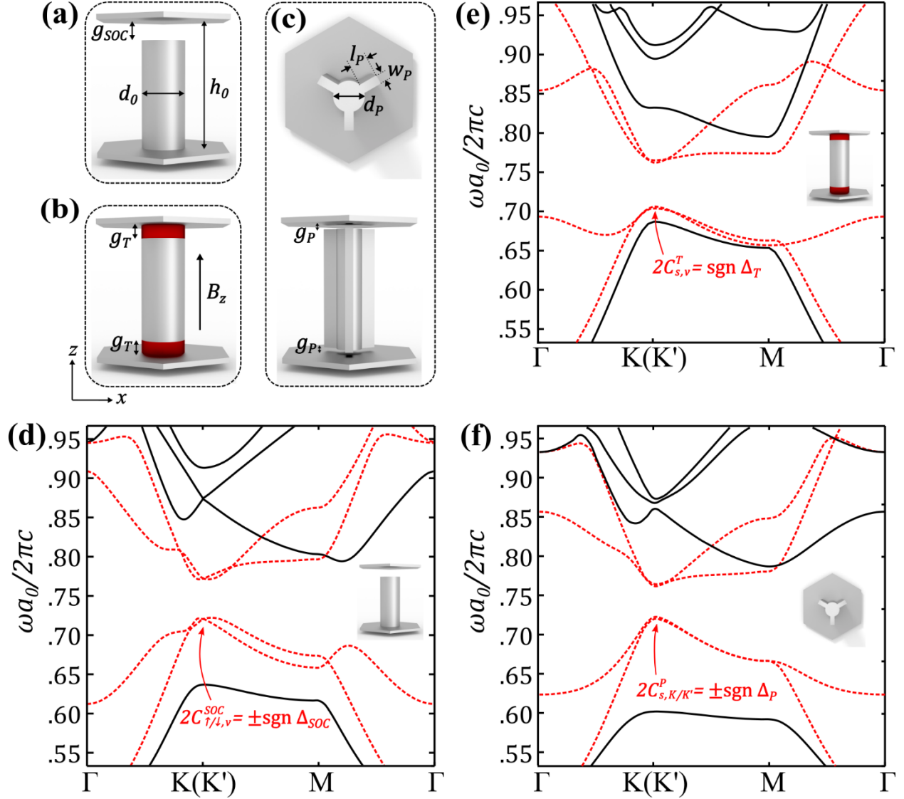
Figure 2: A library of topological phases of light. (a,b,c) The unit cells of the three PTIs emulating QSH, QH, and QVH effects, respectively. In (b), the gyromagnetic material (red disks) has the following constitutive parameters: \epsilon = 1 , \mu_{xx/yy/zz} = 1 , \mu_{xy} = -\mu_{yx} = -i\delta with \delta = 0.8 , and \mu_{ij} = 0 otherwise. (d,e,f) Photonic band structures corresponding to the PTIs in (a,b,c), respectively. The bandgap widths \Delta are proportional to the respective overlap integrals \Delta_{SOC} \propto g_{SOC} , \Delta_T \propto \delta \times g_T , and \Delta_P defined in SM. The local spin-valley Chern indices of the lower bands are listed. Geometric parameters are chosen to ensure spin-degeneracy and approximately equal band gaps: h_0 = a_0 , d_0 = 0.345a_0 , g_{SOC} = 0.15a_0 , g_T = 0.1a_0 , g_P = 0.03a_0 , d_P = 0.2a_0 , l_P = 0.116a_0 , and w_P = 0.06a_0 . The symmetric rod-to-plate gaps in (c) can be filled with low-index spacer for structural stability.
