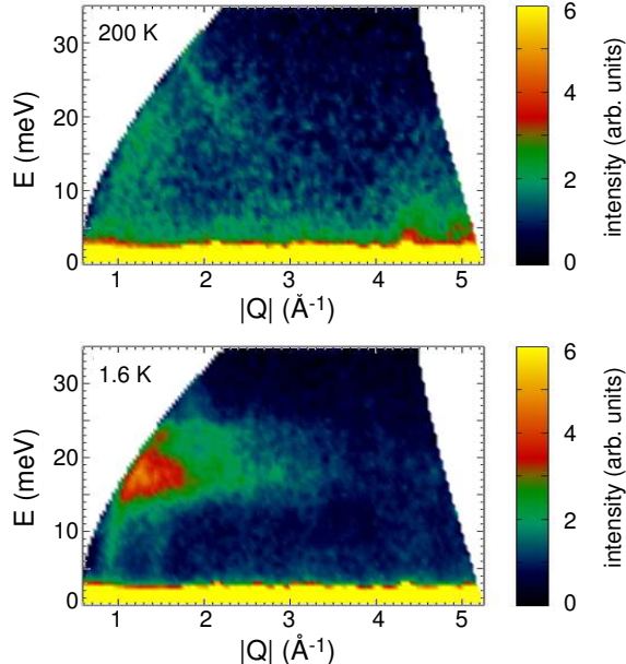
FIG. 7. Contour plots of INS intensity from CrTe 3 powder versus energy and momentum transfer measured at T = 200 K (upper panel) and 1.6 K (lower panel). The data were collected using an incident energy of E_i = 50 meV.
