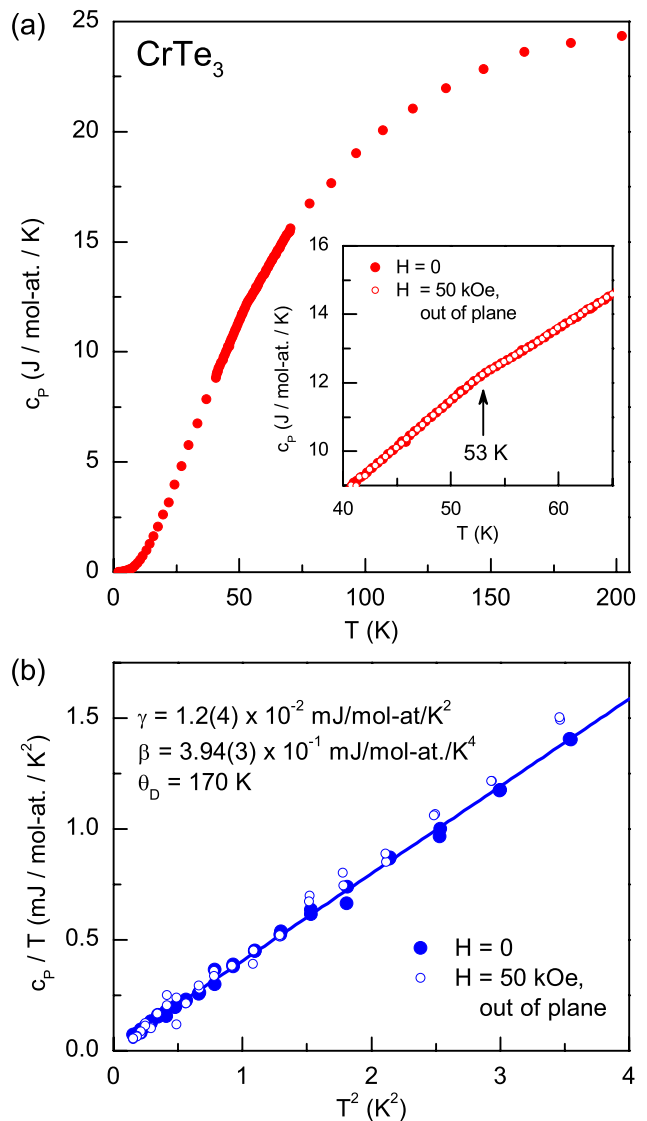
FIG. 4. (a) Heat capacity of a \text{CrTe}_3 single crystal. The weak anomaly observed near 53 K is shown in the inset. (b) Heat capacity between 0.38 and 2 K collected in zero and 5 T magnetic fields showing c_P \propto T^3 behavior. A linear fit to the zero field data is shown and the resulting parameters are listed on the plot.
