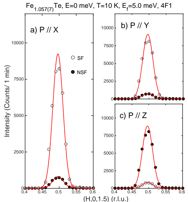
FIG. 4. Polarization analysis of the elastic (0.5, 0, 1.5) magnetic Bragg peak showing spin-flip (open circles) and non-spin-flip (filled circles) scattering with the incident beam of neutrons polarized along the X, Y, and Z directions as defined in the main text. The peak in the non spin-flip channel in panel (a) is the result of incomplete polarization of the neutron beam and is defined by the flipping ratio.
