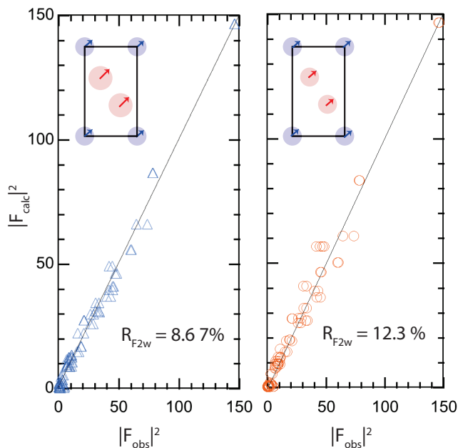
FIG. 8. Results from single magnetic structure refinement on a single crystal of \text{Fe}_{1.141(5)}\text{Te} performed on the HB-3A diffractometer. (a) shows the results of a refinement where the interstitial iron moment sizes were allowed to vary while (b) shows a refinement where they were constrained to be equal. For model (a) the refined size of the Fe moment in the FeTe layers is 2.01(2) \mu_B and 3.5(5) \mu_B on the interstitial site. In model (b), the iron moments in both the FeTe layers and interstitial sites were constrained to be equal giving a refined moment size of 2.1(1) \mu_B .
