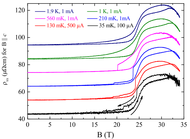
FIG. 3. (Color online) Transverse magnetoresistivity of \text{UPt}_2\text{Si}_2 at various temperatures for B \parallel c axis; for details see text.
