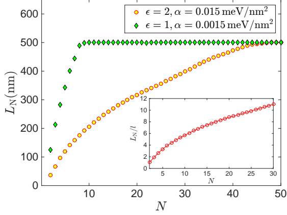
FIG. 12. The 'length' of the Wigner crystal L_N , as a function of the number of charges N , for various potential depths \alpha and dielectric constants. The length of the nanotube is L = 500 nm. Inset: L_N/l for an infinite nanotube with parabolic confinement. L_N/l is a universal function of N .
