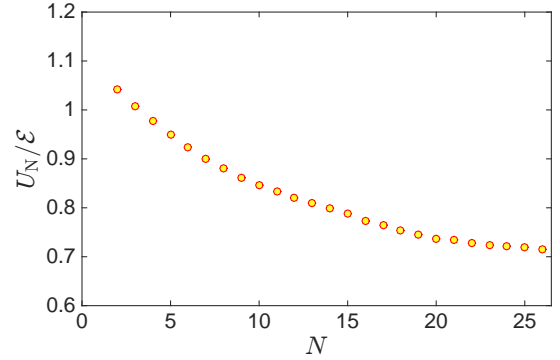
FIG. 11. Dimensionless charging energy as function of the particle number N .
