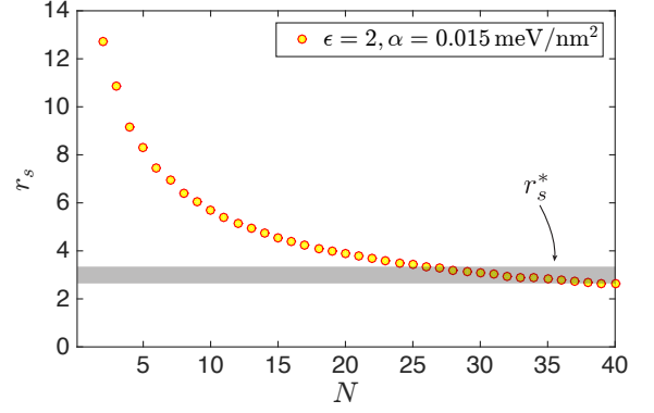
FIG. 13. The dimensionless parameter r_s as a function of the number of charges N in the middle of a 500 nm long nanotube for \alpha = 0.015 meV/nm 2 and \epsilon = 2 . The Wigner crystal starts to melt at the center for N = 26 , once r_s decreases below the crossover value r_s^* \approx 3.3 .
