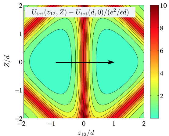
FIG. 3. (Color online) Contour plot of the background potential U_{\text{tot}} in Eq. (10) in terms of relative and center of mass coordinates. Tunneling between the two minima ( z_{12} = \pm d, Z = 0 ) gives rise to the exchange splitting J . The black arrow indicates the semiclassical tunneling path used here.
