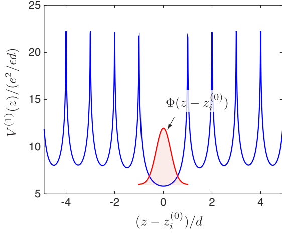
FIG. 9. (Color online) The Hartree potential V_i^{(1)}(z) confining the i 'th electron, defined in Eq. (B6).
