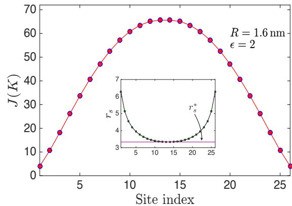
FIG. 7. (Color online) Site dependent exchange couplings for a nanotube with \epsilon = 2 and R = 1.6 nm when N = 26 electrons are confined inside. The inset shows the dimensionless parameter r_s as a function of the site index. Notice that the stability condition r_s \gtrsim r_s^* \approx 3.3 is fulfilled, and the nanotube is in the Wigner crystal regime, though for larger values of N the Wigner crystal is expected to melt at the center of the nanotube.
