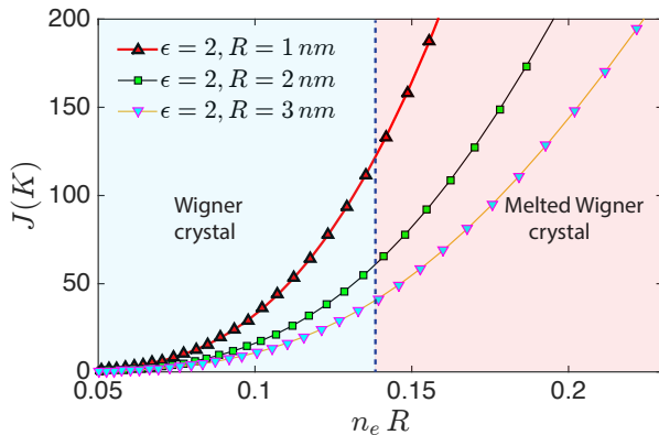
FIG. 4. (Color online) The effective SU(4) spin-isospin exchange coupling J as a function of n_e \cdot R for various nanotube radii with \epsilon = 2 . The vertical dashed line shows the limit of the Wigner crystal regime.
