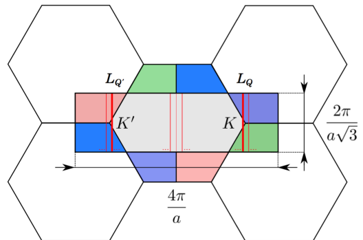
FIG. 8. (Color online) Retailed Brillouin zone (BZ) of graphene (black rectangle). The red lines denote states allowed for a zig-zag carbon nanotube, K and K' mark the two Dirac points, a is the lattice constant. Thick solid red lines indicate the segments L_{\pm Q} .
