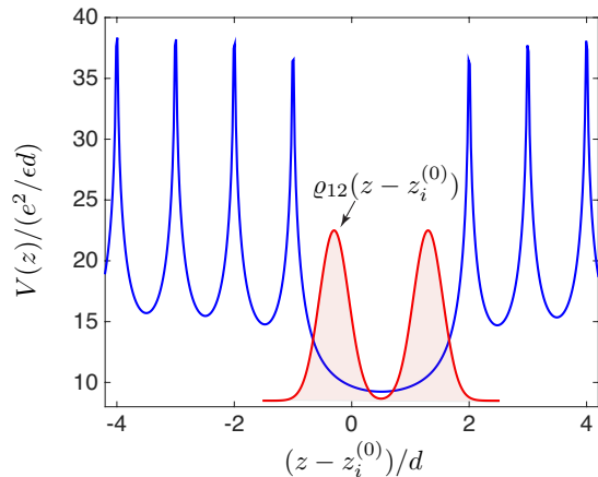
FIG. 2. (Color online) Sketch of the effective potential, V(z) (blue), and the single particle density (red), as obtained from the solution of the two body problem, Eq. (8). d is the distance between two neighboring electrons.
