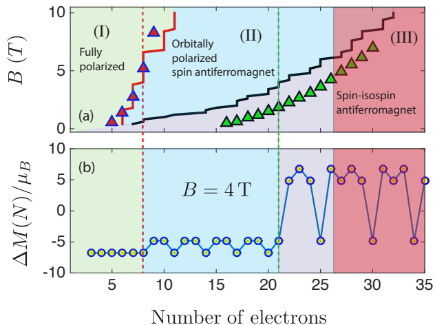
FIG. 1. (Color online) (a) 'Phase diagram' for an unscreened nanotube with \epsilon = 2 and of a radius R = 1.6 nm, as a function of particle number N , and external magnetic field B . Red and black curves denote the phase boundaries based upon our theoretical calculations with spin-orbit coupling, \Delta_{SO} = 0.186 meV ( \Delta_{SO} \approx 2.1 K). The fully polarized, orbitally polarized, and unpolarized states are displayed in different colors. Green and red symbols indicate the boundaries for the experimental 'phase diagram' of Ref. [27]. (b) Overall magnetization change at charge transitions as a function of N for B = 4 T. The vertical dashed lines indicate the jumps corresponding to the phase boundaries. For N > 26 the Wigner crystal starts to 'melt'. The melted region is indicated by the red shaded areas.
