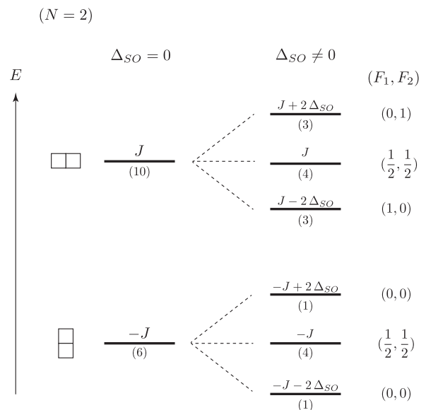
FIG. 5. Energy levels of an N = 2 Wigner molecule, as obtained from exact diagonalization of the effective Hamiltonian. On the l.h.s., the \Delta_{\text{SO}} = 0 spectrum is shown, with states classified by SU(4) representations, indicated by the Young-tableaux. For \Delta_{\text{SO}} \neq 0 states are classified in terms of the residual \text{SU}(2) \times \text{SU}(2) symmetry.
