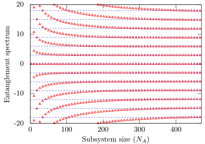
FIG. 5. The single-particle entanglement spectrum of the SSH model with PBC in its topologically non-trivial phase ( \delta t = -0.01 ). The blue dotted lines are guide for eyes. Each level is doubly degenerate.
