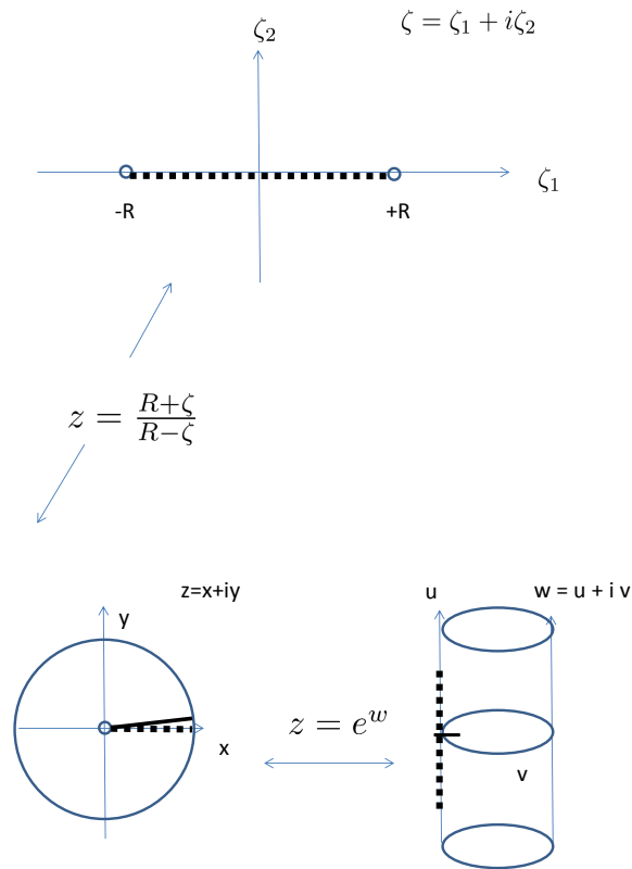
FIG. 2. Conformal Map
