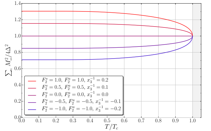
FIG. 4: Deviation of Nambu's Sum from polarization corrections to the J = 2 Higgs modes of {}^3\text{He-B} for a range of interactions in both the Landau and Cooper channels.
