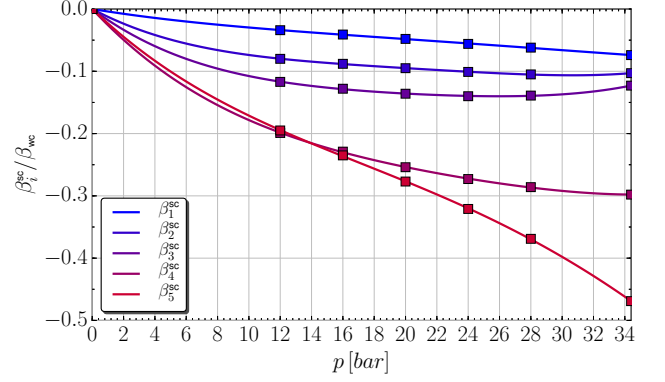
FIG. 1: Strong-coupling corrections to the GL \beta parameters interpolated from the results of Ref. 27 [data squares]. The \beta_i^{\text{sc}} are extrapolated below P = 12 bar to weak-coupling ( \beta_i^{\text{sc}} = 0 ) at p = 0 bar.
