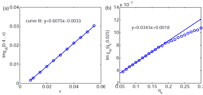
FIG. 8. Numerical calculations of the surface dynamical susceptibility of charge neutral nodal-loop semimetals with nearly completely filled surface bands: (a) the frequency dependence at q_{\parallel} = 0.4 , and (b) the wavevector dependence at \nu = 0.025 .
