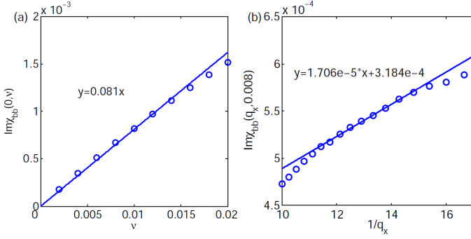
FIG. 7. Numerical calculations of the surface dynamical susceptibility of slightly hole-doped nodal-loop semimetals with partially filled surface bands: (a) frequency dependence at q_{\parallel} = 0 ; and (b) wavevector dependence at \nu = 0.008 . Note the horizontal axis in (b) is 1/q_x .
