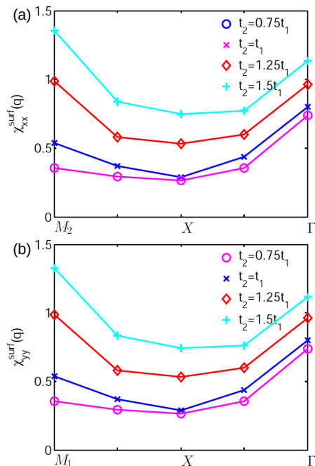
FIG. 5. Wavevector dependence of the surface-mode in-plane spin susceptibilities for different t_2 values at fixed U = 0.5t_1 , (a) \chi_{xx} , and (b) \chi_{yy} . The high-symmetry points M_1 = (\pi, 0) , M_2 = (0, \pi) , X = (\pi, \pi) , and \Gamma = (0, 0) .
