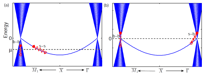
FIG. 6. Schematic illustration of different types of electron-hole excitations that couple to surface spins. (a) When the surface bands are partially filled. (b) When the surface bands are (nearly) completely filled. The electron-hole excitations purely from the surface (bulk) states are denoted by “ s-s ” (“ b-b ”); while the process of creating a hole in the surface states and an electron in the bulk states is denoted by “ s-b ”.
