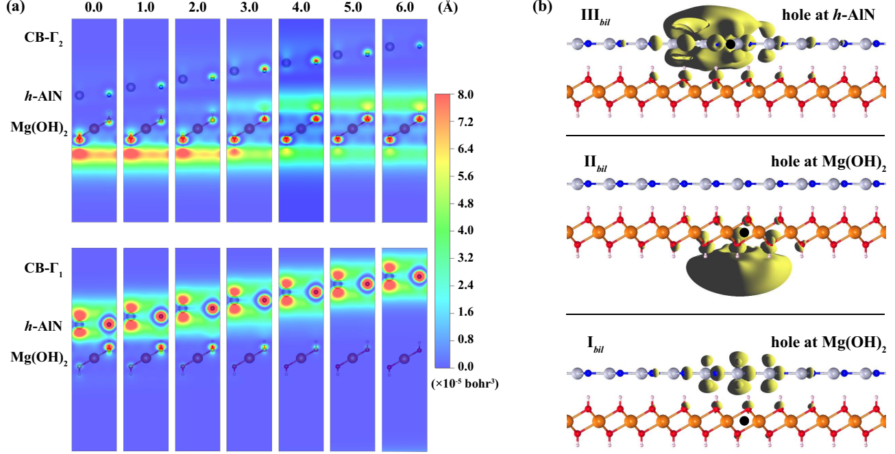
FIG. 5: (Color online) (a) Layer-layer distance dependent band decomposed charge densities at the \Gamma point for the lowest two bands (CB- \Gamma_1 and CB- \Gamma_2 ) are presented. The the numbers on the upper part of the figure are distances between the layers in the unit of \text{\AA} . The optimized layer-layer distance is set to 0.0 \text{\AA} . (b) shows the wave function of the lowest three excitons which are labeled as \text{I}_{bil} , \text{II}_{bil} , and \text{III}_{bil} . The yellow regions are the probability of the electron localization when the hole is at a specific point. The position of holes are shown as a black point on the structures for all wave functions. The methodology for the determination of excitonic wave functions is given in Appendix B.
