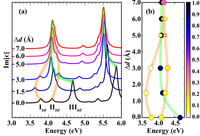
FIG. 4: (Color online) (a) The imaginary part of the dielectric functions of the AB' stacked heterobilayer are shown for different interlayer distances starting from ground state distance of 2.13 \text{ \AA} . \Delta d refers to interlayer distance while the ground state distance is set to 0 and labeled as 0.0 \text{ \AA} . The lowest three exciton peaks are labeled as \text{I}_{bil} , \text{II}_{bil} , and \text{III}_{bil} . (b) The distance dependent oscillator strengths of lowest three excitons are shown. Color code is given. The position of the prominent peaks are illustrated by shaded curves. The length of the out-of-plane lattice vector is fixed for different interlayer distance.
