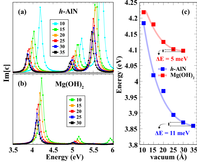
FIG. 7: (Color online) The results of vacuum spacing tests: (a) and (b) The imaginary part of the dielectric functions of the monolayer h -AlN and \text{Mg}(\text{OH})_2 for different vacuum spacing values, respectively. (c) The first exciton peak positions are shown. The blue and red curves correspond to the monolayer h -AlN and \text{Mg}(\text{OH})_2 , respectively.
