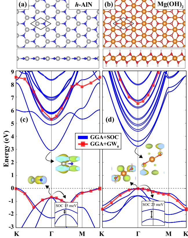
FIG. 1: (Color online) Upper panel illustrates the structure of monolayer h -AlN (left) and \text{Mg}(\text{OH})_2 (right). (a) and (b) are the structures (top and side view), the solid black parallelograms show the unitcell of the structural, (c) and (d) are the band structures of h -AlN and \text{Mg}(\text{OH})_2 , respectively. The blue and light-red curves with square are for GGA+SOC and GGA+ \text{GW}_0 , respectively. The dashed vertical line is shows the Fermi energy. In the band diagram, the charge densities of the VBM and CBM and the spin-orbit splitting at the \Gamma point.
