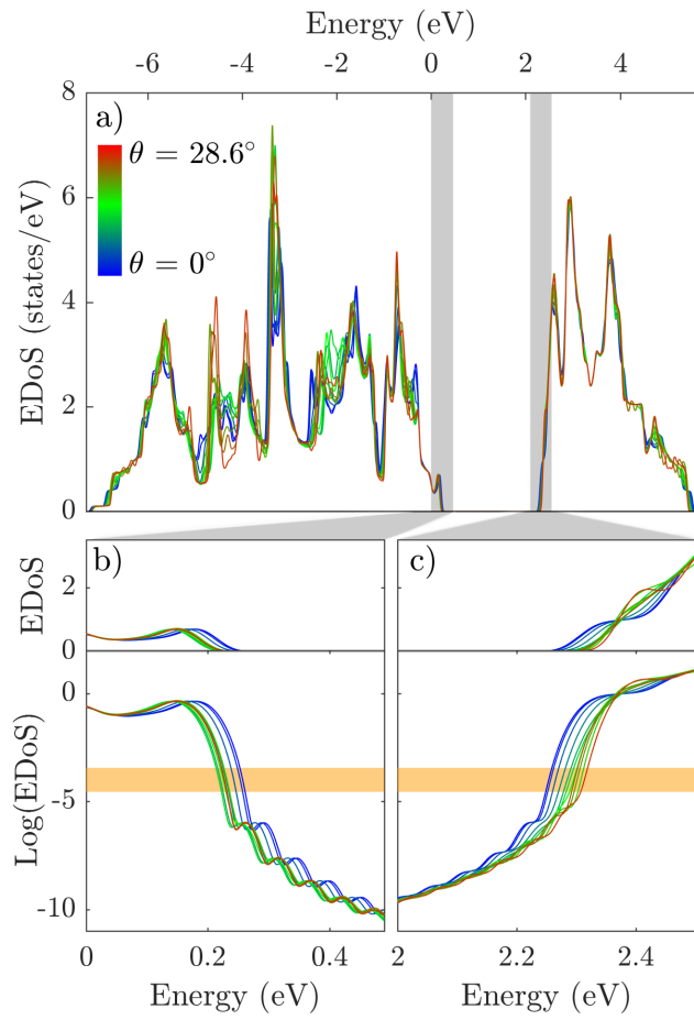
FIG. 4. (a) EDoS for twisted bilayer MoS 2 from 0^\circ (blue) to 28.65^\circ (red) twist angle. (b) and (c) EDoS near the valence and conduction band extrema, with the logarithmic scales showing the changes in greater detail. These calculations use a disk cut-off radius R = 300 \text{ \AA} (193,700 atoms) and are averaged over 100 configurations across the unit-cell ( 10 \times 10 grid).
