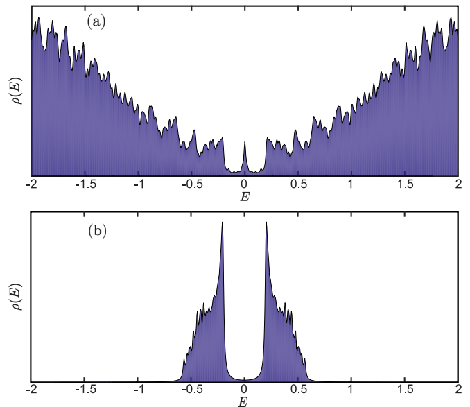
FIG. 4. The density of state plots for a Weyl loop chiral superconductor [Panel (a)] and a 2D p+ip SC with a flat band dispersion [Panel (b)], both in the “strong” pairing phase and with a vortex configuration. The spikes at high energies are due to finite-size effects (the system size is 20 \times 20 \times 10 for four bands). For both Hamiltonians, there exists a bulk gap at \mu = 0.2 (in unit of hopping parameters), however the clear distinction is that there exist in-gap states for the Weyl loop surface SC.
