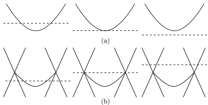
FIG. 3. Panel (a): A process to deform the weak pairing phase into strong pairing phase in 2D p+ip SC, where the dashed lines are the chemical potential. It necessarily involves a gap closing at \mathbf{k} = 0 , where the SC order parameter is forced to vanish by fermionic statistics. Panel (b): The corresponding process for the drumhead surface SC, shown at a given \theta . No gap closing is involved with SC order turned on. In the last figure the drumhead dispersion can be further distorted.
