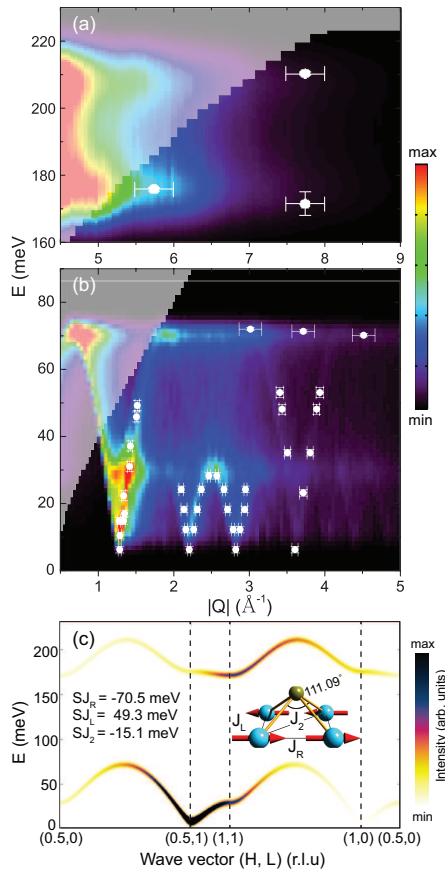
FIG. 3: Comparisons between the SpinW simulated spin excitation spectra and experimentally determined dispersion relations (white points) for BaFe 2 S 3 . (a) Instrumental resolutions of 13.3 meV and (b) 5 meV have been convolved for comparison with the powder averaged experimental data in Figs. 2(a)-2(d). The white shaded areas are experimentally inaccessible with E_i = 250 meV. (c) SpinW simulated spin excitations along high symmetry directions in the [H, L] 2D Brillouin zone for single crystals with the parameters labeled on the figures. The other parameters, SJ_7 and SJ_s , have been fixed at 3.0 and 0.1 meV, respectively. The color represents intensities. We convolve a constant 5 meV instrumental resolution for visualization. The inset in panel (c) shows a tetrahedron and associated exchange interactions.
