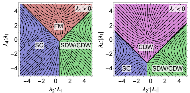
FIG. 6: RG phase diagram showing a leading instability as a function of initial coupling constants. The figure on the left shows the case of positive \lambda_1 > 0 , while the one on the right corresponds to \lambda_1 < 0 . ( \lambda_1 never changes sign under the RG flow.) There are four possible instabilities: SC superconducting, ferromagnetic (FM), charge-density-wave (CDW) and a competing spin/charge-density-wave (SDW/CDW). The Hubbard model initial conditions \lambda_1 = \lambda_2 = \lambda_4 > 0 lead to the development of FM instability.
