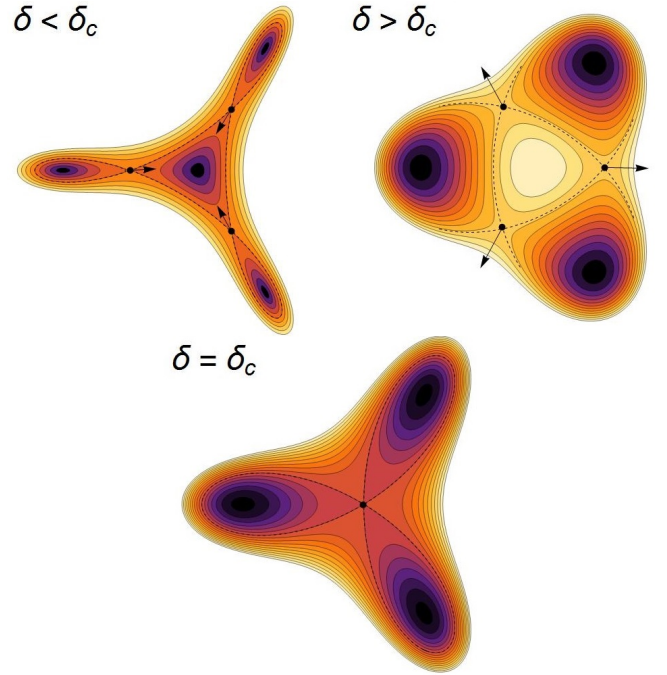
FIG. 1: Pictorial representation of Fermi surface families in a biased bilayer graphene system for three different values of the interlayer voltage bias \delta . Three van Hove saddles with dispersions \propto (p_x^2 - p_y^2) are shown with black dots ( \delta \neq \delta_c ) while arrows indicate their displacement upon increasing the value of \delta . At the critical value of the bias \delta_c they merge into a monkey saddle \propto (p_x^3 - 3p_x p_y^2) that closes into a trifolium-shaped Fermi surface.
