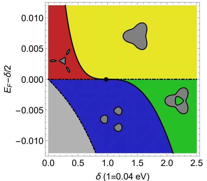
FIG. 2: There are four phases with different Fermi surface topologies in biased bilayer graphene. They are separated by two lines of phase transitions, one of a band-edge type (dash-dotted) and the other of the van Hove or equivalently a neck-narrowing type (solid). The multicritical Lifshitz point is located at the crossing of these two lines. In the gray area the Fermi level lies within the gap with no FS. Note different scales for the voltage \delta and the Fermi energy E_F .
