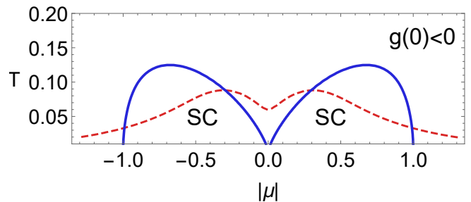
FIG. 5: Phase diagram (blue solid line) for an isolated monkey saddle and attractive coupling constant. Critical chemical potential is determined by the equation |g_0|\nu(\mu_c) = 2 and the plot is given in units of \mu_c for both temperature and chemical potential. Any odd saddle ( n = 3, 5, \dots ) has qualitatively same phase diagram, but the situation is different for even saddles ( n = 2, 4, \dots ). Even case is illustrated with red dashed line for n = 4 .
