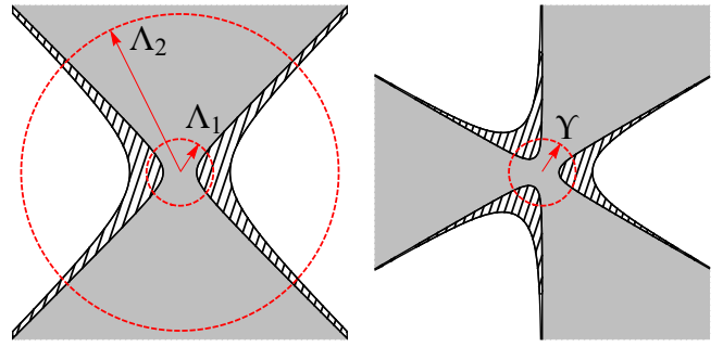
FIG. 4: Left : A Fermi surface near a van Hove saddle calls for a two-cutoff RG scheme. The grey area represents occupied electron states. The hatched region of the phase space corresponds to a step d\xi in electron energy. Normally, one cutoff d\Lambda_1 \sim d\xi is sufficient, but here we see that the logarithmic DoS at the van Hove saddle together with an open hyperbolic Fermi surface lead to tails of the hatched region that reach out to the rest of the Fermi surface away from the van Hove saddle. The purpose of the second cutoff \Lambda_2 is to cut these tails and isolate van Hove saddle.
