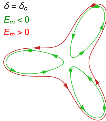
FIG. 3: Quasi-classical LL orbits in momentum space for energies slightly below and slightly above the monkey saddle (and critical voltage bias). The number of connected FS components changes from three to one as the Fermi level crosses zero.
