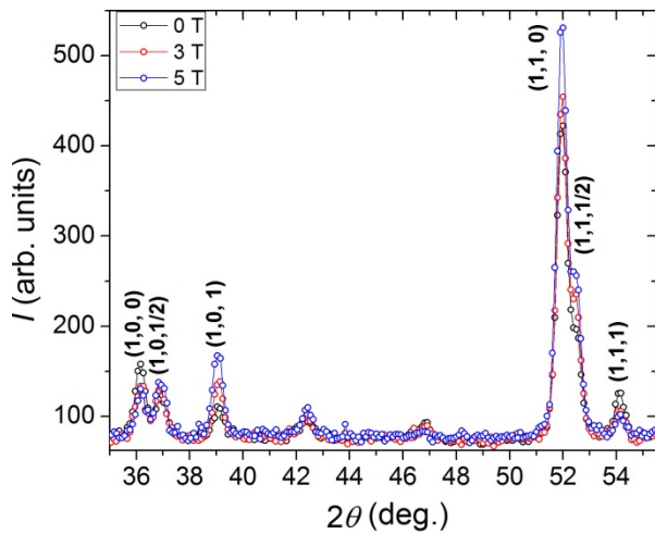
FIG. 9. Part of the neutron powder diffraction patterns of \text{La}_{0.25}\text{Pr}_{0.75}\text{Co}_2\text{P}_2 collected at 3 K under applied magnetic fields 0, 3, and 5 T.
