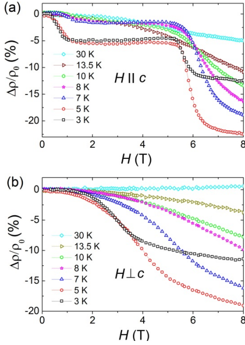
FIG. 5. Magnetoresistance measured on a single crystal of \text{La}_{0.25}\text{Pr}_{0.75}\text{Co}_2\text{P}_2 at various temperatures with the magnetic field applied parallel (a) and perpendicular (b) to the c axis.
