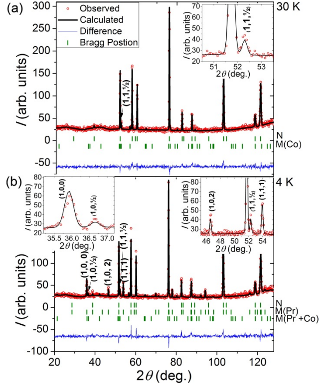
FIG. 6. Rietveld refinement of neutron powder diffraction patterns of \text{La}_{0.25}\text{Pr}_{0.75}\text{Co}_2\text{P}_2 collected at 30 K (a) and 4 K (b). Magnetic peaks are emphasized in the insets.
