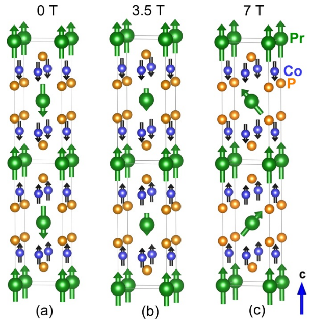
FIG. 12. Refined magnetic structure of \text{PrCo}_2\text{P}_2 with applied magnetic fields up to 7 T at 1.5 K.
