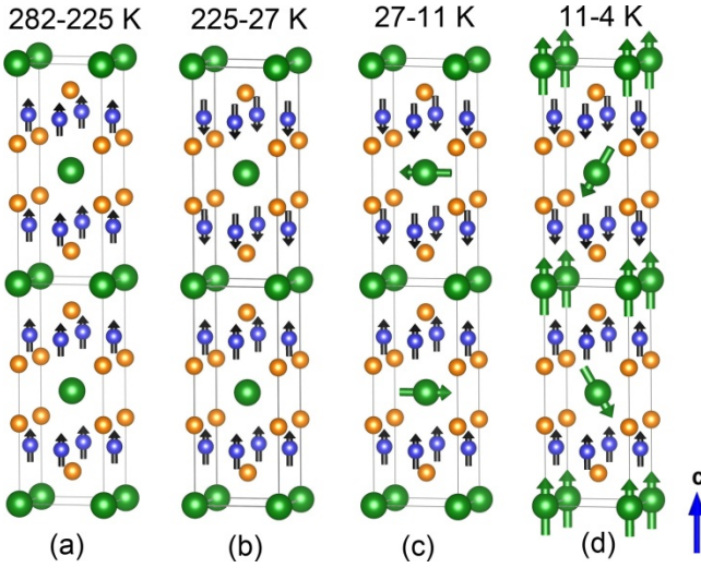
FIG. 7. Evolution of the magnetic structure of \text{La}_{0.25}\text{Pr}_{0.75}\text{Co}_2\text{P}_2 as a function of temperature: (a) 282-225 K, (b) 225-27 K, (c) 27-11 K, and (d) 11-4 K.
