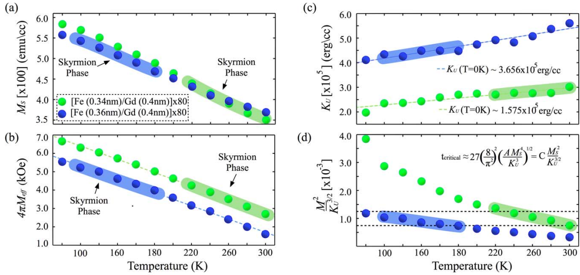
Figure 4. Temperature dependent magnetic and ferromagnetic resonance properties. The magnetization (a), effective magnetization (b), uniaxial anisotropy (c) and the ratio (d) are shown for [Fe (0.34nm)/Gd (0.4nm)]x80 and [Fe (0.36nm)/Gd (0.4nm)]x80. The region in temperature where each Fe/Gd film exhibits a skyrmion phase has been shaded to serve as a guide to the eye. By linearly fitting the uniaxial anisotropy with temperature, we can conclude that K_U is positive at absolute-zero (c). The enclosed region with dashed lines in (d) represents a window of values where both Fe/Gd films exhibit a skyrmion phase.
