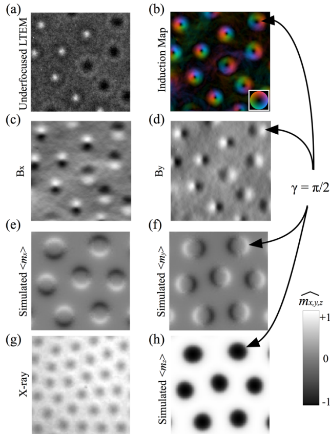
Figure 6. Comparison between numerical and experimental observation of skyrmions. (a, b) Under-focused Lorentz-TEM image and its corresponding magnetic induction map illustrate the Bloch-line arrangement of the skyrmions. (c, d) The individual in-plane components of the magnetic induction B_x and B_y are obtained from (b). (e, f) Detail a numerical computed average magnetization across the slab for \langle m_x \rangle and \langle m_y \rangle . (g) A transmission X-ray microscopy of the skyrmion phase solely shows the presence of cylindrical domains which resembles the average magnetization across the slab for \langle m_z \rangle in (h). A skyrmion with S = 1 , \gamma = \pi/2 is referenced to directly compare experimental and numerical results in (b, d, f, h). The scale bar references the micromagnetic domain states.
