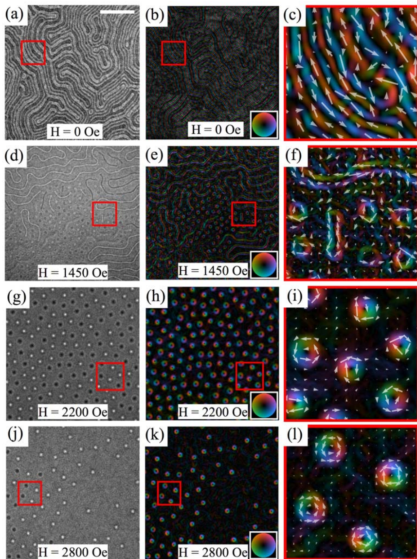
Figure 1. Real space imaging of the field-dependent magnetic domain morphology of [Fe (0.34 nm)/Gd (0.4 nm)] x80 . Under-focused Lorentz TEM images (first column) measured at room temperature and their corresponding magnetic induction color maps (second column) are detailed. The images are captured as a perpendicular magnetic field is applied from zero-field to magnetic saturation. Four different magnetic states are observed as the field is swept, including:
