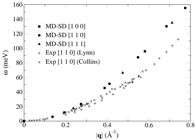
FIG. 8. Transverse magnon dispersion relations at T = 300 K obtained from MD-SD simulations for L = 16 . The experimental results reported by Lynn [61] and Collins [62] for the [1\ 1\ 0] direction are also plotted for comparison.
