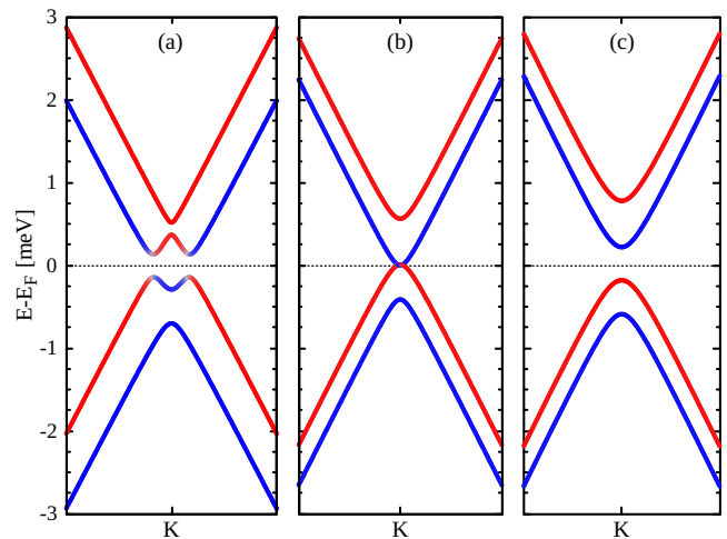
FIG. 1. (Color online) Typical band structure of effective model near the K valley. Left panel shows an 'inverted band' regime, with strong spin mixing of the different states, as indicated by the red/blue shading, and typical of |S_1 + S_2| > \Delta . Middle panel shows a spin split semimetallic phase, while right panel shows a 'direct band' regime where a finite bulk gap develops with nearly full spin polarization, obtained when |S_1 + S_2| < \Delta .
