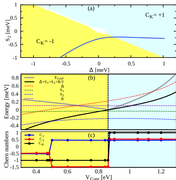
FIG. 4. (Color online) (a) Phase diagram for Graphene-TMD system in Eq. 1 in the S_2 - \Delta projection with R = 0.1 meV, and S_1 \in [-0.16, 0.16] meV. Trivial insulating phase in yellow C_K = -1 , and mass inverted phase in blue C_K = +1 , divided by the semimetallic phase, white curve. Blue line shows the line cut for graphene-MoS 2 system as a function of V_{Gate} . (b) Gate voltage dependence of effective Hamiltonian parameters used to fit the tight-binding band structure results. Black line shows evolution of band gap, which closes at V_{Gate} = 0.86 eV. For V_{Gate} < 0.86 eV, in the inverted band regime, spin orbit contribution dominates over the staggered term, given approximately by \Delta + S_1 + S_2 < 0 , slightly shifted by Rashba term. In the opposite regime, staggered potential dominates and creates a trivial band gap. (c) Chern numbers for K valley, as in (a). Switch near V_{Gate} = 0.5 eV is due to a band crossing at the K point, while jump at V_{Gate} = 0.86 eV indicates gap closing that separates inverted mass regime from direct band regime. V_{Gate} = 0 corresponds to graphene Dirac point 20 meV higher than the top valence band in MoS 2 .
