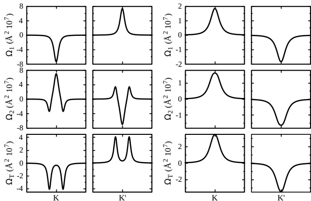
FIG. 2. Berry curvature \Omega_n at K and K' valleys for both inverted and direct band gap regimes. Left two columns show results for the inverted band regime corresponding to Fig. 1a. Right two columns are for the direct band regime corresponding to Fig. 1c. Upper (middle) plots describe Berry curvature of the lowest (highest) energy valence bands in Fig. 1, n = 1(2) . Lower plots show the total valence band Berry curvature, \Omega_T = \Omega_1 + \Omega_2 . The different Berry curvature distribution between K and K' is evident in both cases.
