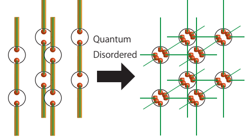
FIG. 5: (Color online) Thick orange lines depict an array of (1+1)d O(4) NL\sigma models with WZ terms at level k_{\text{eff}} = 4S/3 , which are placed in the background of a prefixed \text{VBS}_z order (green lines) - see text for details. Condensation of monopoles results in a 3d AKLT-like state on the cubic lattice.
