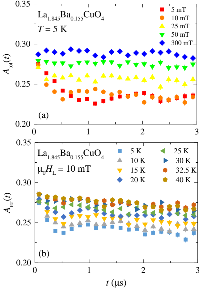
FIG. 7: (Color online) (a) LF- \mu SR time spectra A_{tot}(t) of LBCO-0.155 recorded at T = 5 K and p = 0.83 GPa with different magnetic fields applied along the initial direction of the muon-spin polarization. (b) LF- \mu SR spectra A_{tot}(t) of LBCO-0.155 taken in an applied longitudinal field of \mu_0 H_L = 10 mT for various temperatures ( 5 \text{ K} \leq T \leq 40 \text{ K} ).
