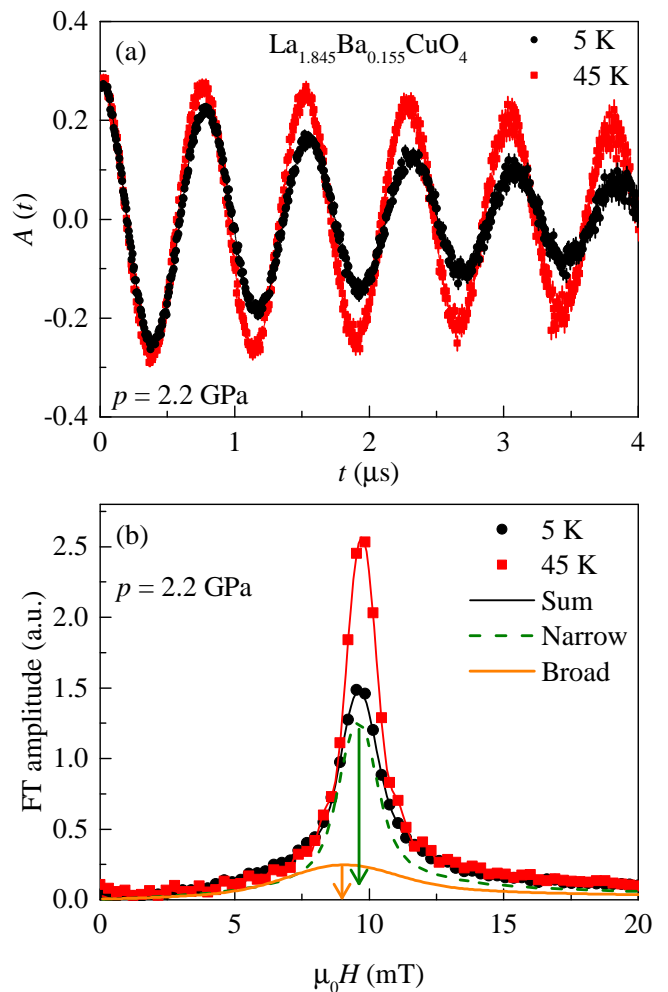
FIG. 10: (Color online) Transverse-field (TF) \mu\text{SR} time spectra A(t) (a) and the corresponding Fourier transforms (FTs) (b) of LBCO-0.155. The spectra were obtained at p = 2.2 \text{ GPa} above (45 K) and below (5 K) T_c (after field cooling the sample from above T_c ). The solid lines in panel (a) represent fits to the data by means of Eq. (4). The solid lines in panel (b) are the FTs of the fitted time spectra. The arrows indicate the first moments for the signals of the pressure cell (green) and the sample (orange), respectively.
