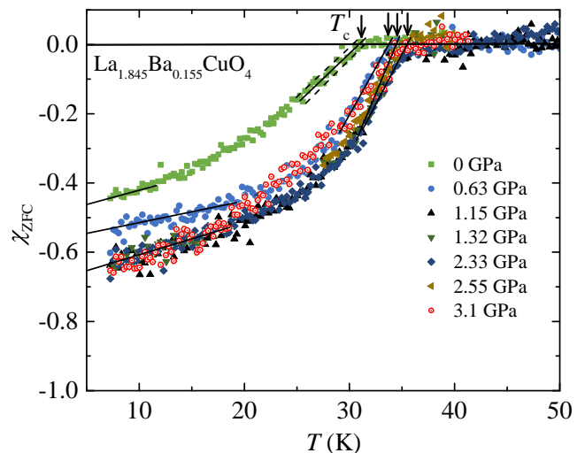
FIG. 5: (Color online) Diamagnetic susceptibility \chi_{\text{ZFC}} of LBCO-0.155 as a function of temperature and pressure. The dependence was measured at ambient and at various applied hydrostatic pressures in a magnetic field of \mu_0 H = 0.5 mT. The arrows denote the superconducting transition temperature T_c .
