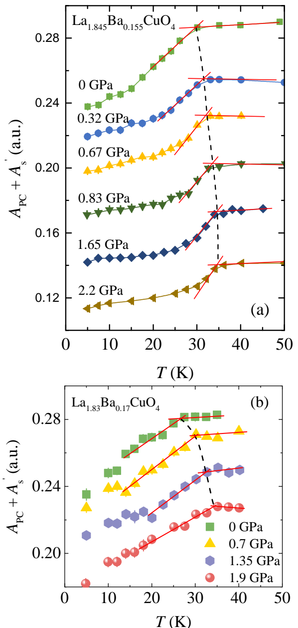
FIG. 9: (Color online) TF asymmetry A'_S for LBCO-0.155 (a) and LBCO-0.17 (b) as a function of temperature for ambient and selected applied pressures in an applied field of \mu_0 H = 3 \text{ mT} . The onset temperature to the magnetically ordered state T_{so} is defined as the temperatures where the linearly extrapolated low and high temperature data points intersect (indicated by the straight lines). The solid curves are guides to the eye.
