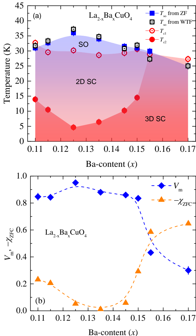
FIG. 4: (Color online) (a) The static spin-stripe order temperature T_{\text{so}} and the SC transition temperatures T_{\text{c1}} and T_{\text{c2}} as a function of Ba-content x in \text{La}_{2-x}\text{Ba}_x\text{CuO}_4 , as determined from ZF- \mu SR, WTF- \mu SR, and magnetization experiments. (b) The magnetic volume fraction V_m and the diamagnetic susceptibility \chi_{\text{ZFC}} as a function of Ba-content x in \text{La}_{2-x}\text{Ba}_x\text{CuO}_4 .
