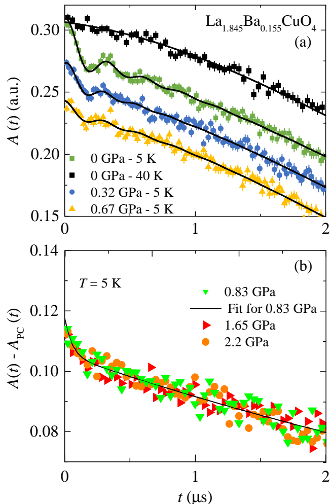
FIG. 6: (Color online) (a) ZF \mu SR time spectra A(t) for LBCO-0.155 recorded at 5 K in the pressure range of 0 \leq p \leq 0.67 GPa. The \mu SR time spectrum at 40 K for 0 GPa is also shown. (b) \mu SR time spectra for LBCO-0.155 after subtracting the pressure cell contribution from the total signal, A_S(t) = A(t) - A_{PC}(t) , recorded at 5 K in the pressure range 0.83 \leq p \leq 2.2 GPa. The solid lines represent fits to the data by means of Eq. (1).
