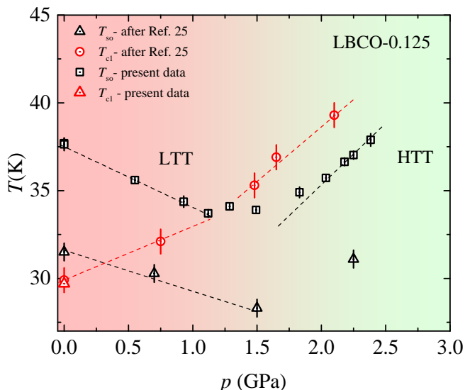
FIG. 16: (Color online) Pressure dependence of T_{so} and T_{cl} for LBCO-1/8, taken from weak-transverse field \mu SR and magnetization data. The terms LTT and HTT stand for the low-temperature tetragonal and high-temperature tetragonal structural phases.
